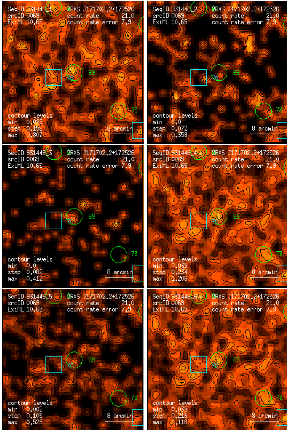
Figure 69: RASS 931446: detection 0069: band rate images, Gaussian filter: (1) PSPC channels 11 – 41, (2) 52 – 90, (3) 91 – 201, (4) 11 – 235, (5) 52 – 201, (6) 11 – 201. Broad band rates in counts/ks. Band rate contour levels in counts/ks/arcmin 2 .
