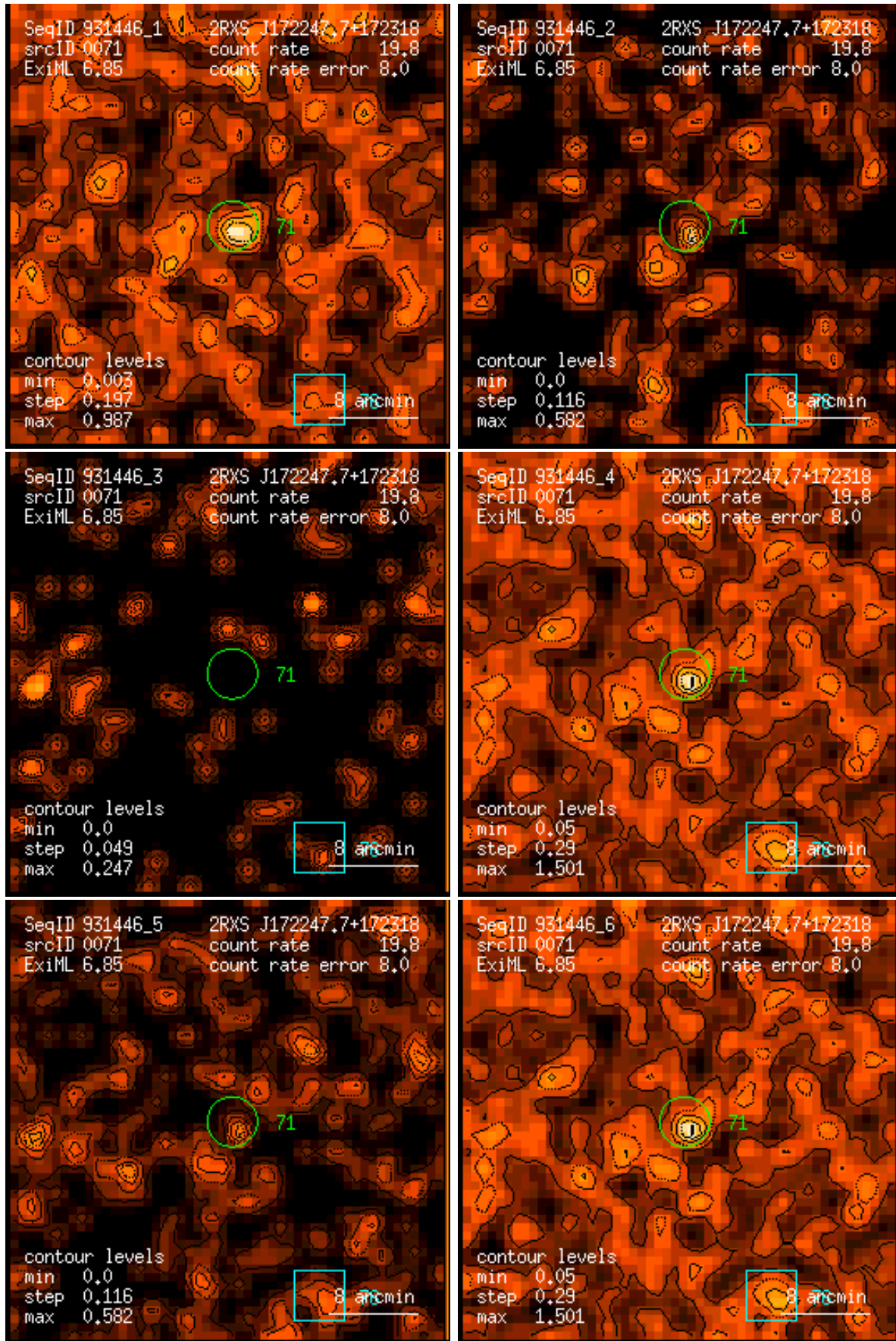
Figure 71: RASS 931446: detection 0071: band rate images, Gaussian filter: (1) PSPC channels 11 – 41, (2) 52 – 90, (3) 91 – 201, (4) 11 – 235, (5) 52 – 201, (6) 11 – 201. Broad band rates in counts/ks. Band rate contour levels in counts/ks/arcmin 2 .
