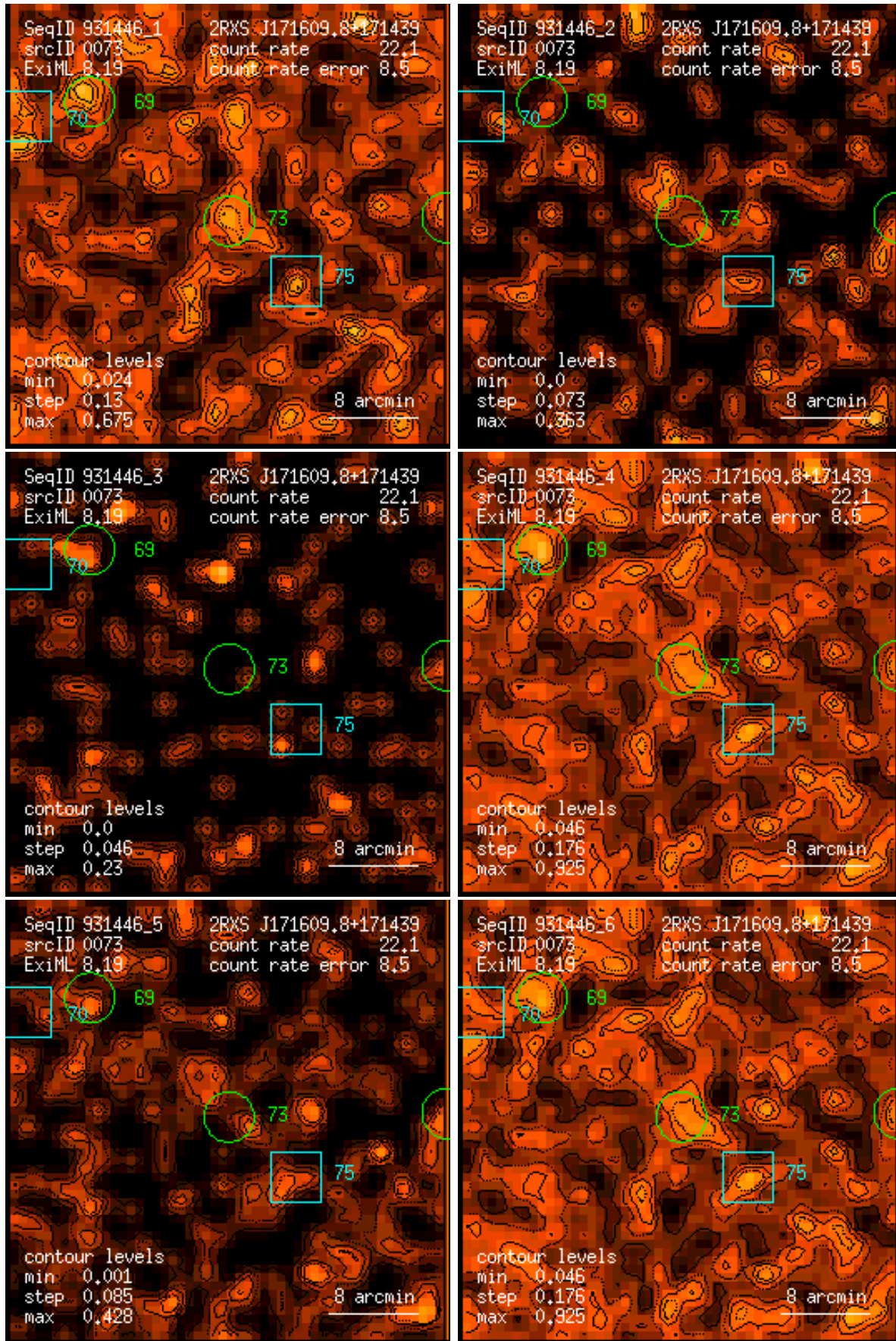
Figure 73: RASS 931446: detection 0073: band rate images, Gaussian filter: (1) PSPC channels 11 – 41, (2) 52 – 90, (3) 91 – 201, (4) 11 – 235, (5) 52 – 201, (6) 11 – 201. Broad band rates in counts/ks. Band rate contour levels in counts/ks/arcmin 2 .
