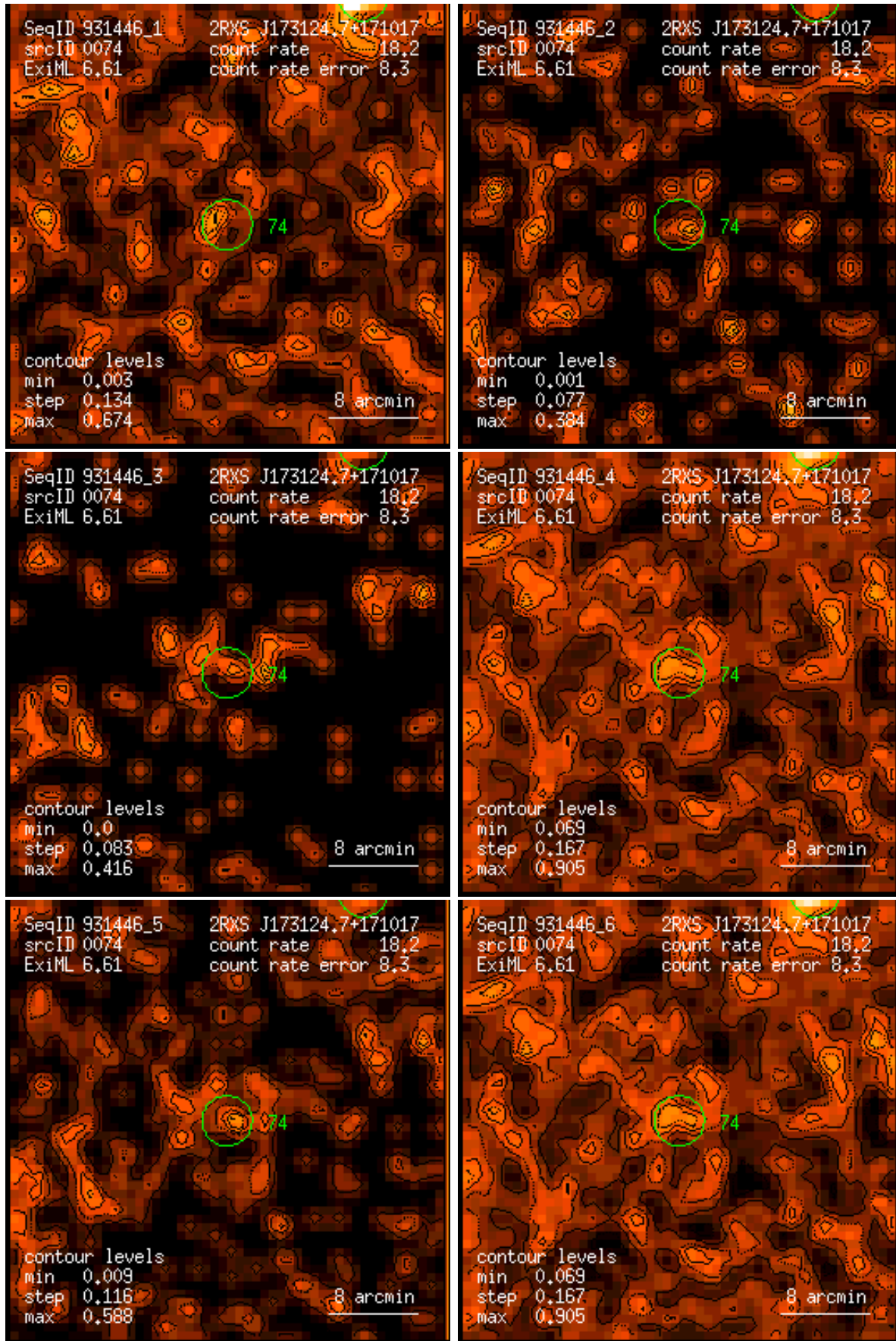
Figure 74: RASS 931446: detection 0074: band rate images, Gaussian filter: (1) PSPC channels 11 – 41, (2) 52 – 90, (3) 91 – 201, (4) 11 – 235, (5) 52 – 201, (6) 11 – 201. Broad band rates in counts/ks. Band rate contour levels in counts/ks/arcmin 2 .
