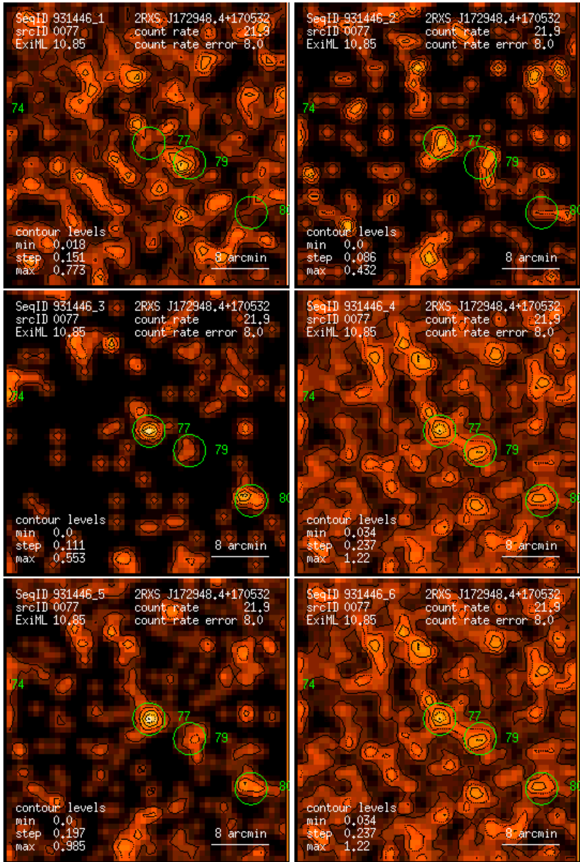
Figure 77: RASS 931446: detection 0077: band rate images, Gaussian filter: (1) PSPC channels 11 – 41, (2) 52 – 90, (3) 91 – 201, (4) 11 – 235, (5) 52 – 201, (6) 11 – 201. Broad band rates in counts/ks. Band rate contour levels in counts/ks/arcmin 2 .
