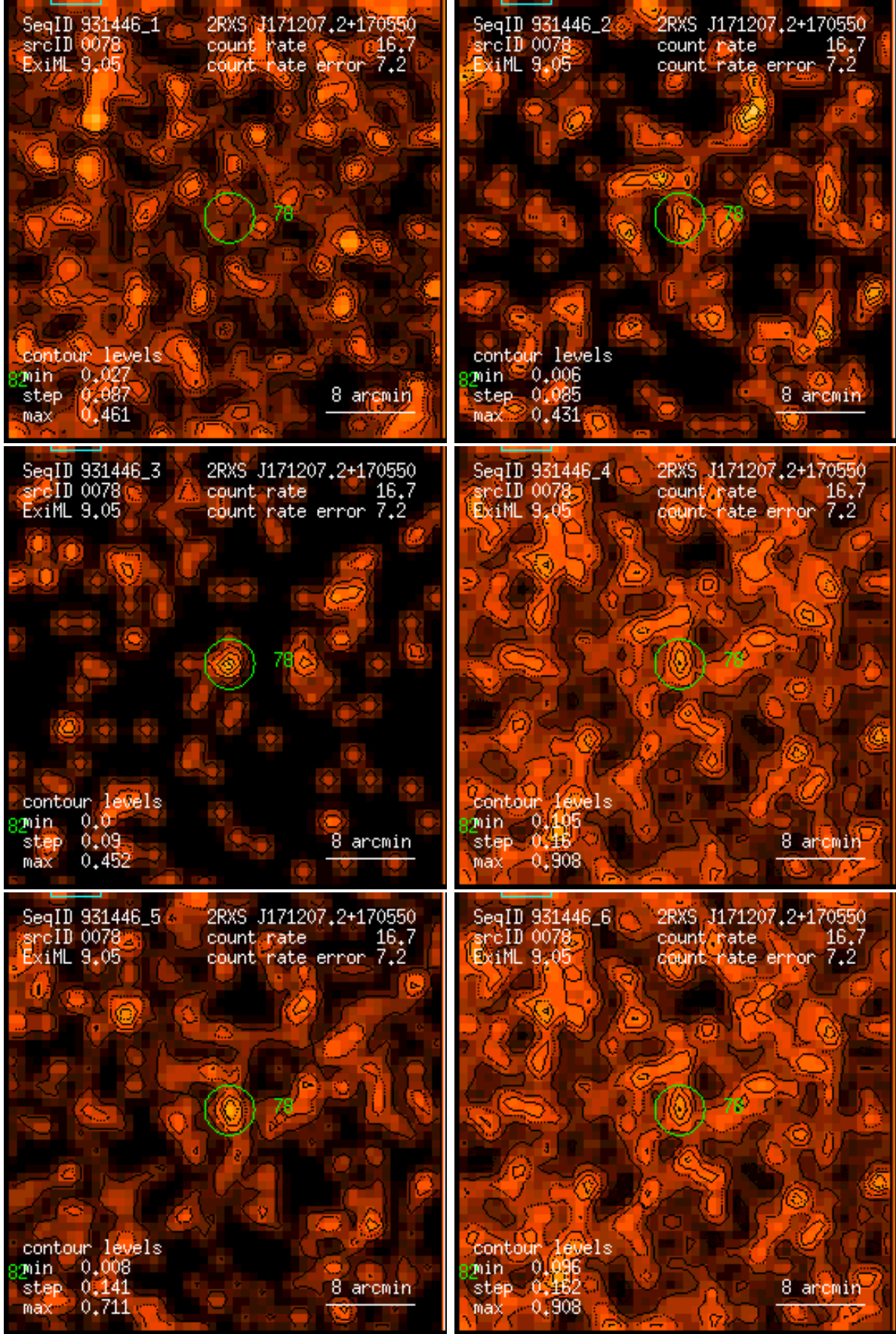
Figure 78: RASS 931446: detection 0078: band rate images, Gaussian filter: (1) PSPC channels 11 – 41, (2) 52 – 90, (3) 91 – 201, (4) 11 – 235, (5) 52 – 201, (6) 11 – 201. Broad band rates in counts/ks. Band rate contour levels in counts/ks/arcmin 2 .
