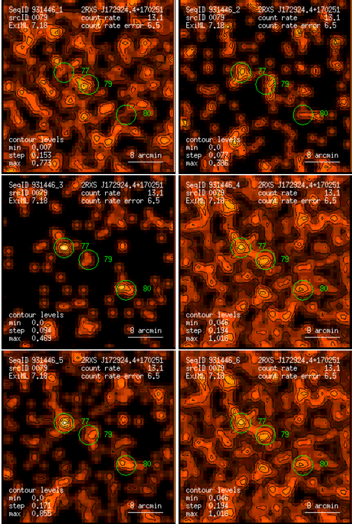
Figure 79: RASS 931446: detection 0079: band rate images, Gaussian filter: (1) PSPC channels 11 – 41, (2) 52 – 90, (3) 91 – 201, (4) 11 – 235, (5) 52 – 201, (6) 11 – 201. Broad band rates in counts/ks. Band rate contour levels in counts/ks/arcmin 2 .
