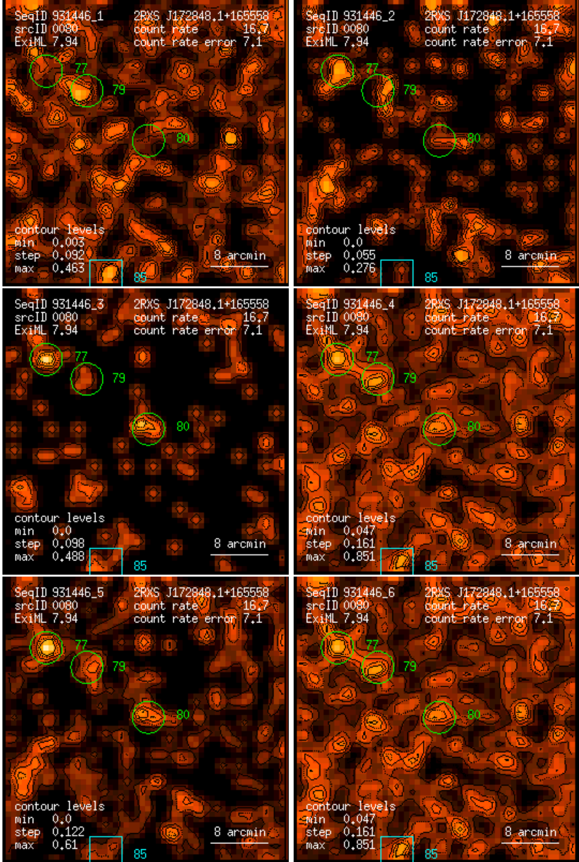
Figure 80: RASS 931446: detection 0080: band rate images, Gaussian filter: (1) PSPC channels 11 – 41, (2) 52 – 90, (3) 91 – 201, (4) 11 – 235, (5) 52 – 201, (6) 11 – 201. Broad band rates in counts/ks. Band rate contour levels in counts/ks/arcmin 2 .
