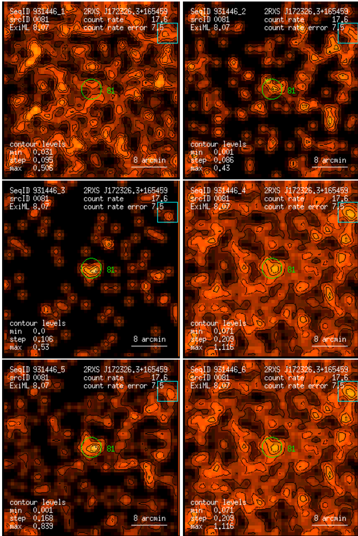
Figure 81: RASS 931446: detection 0081: band rate images, Gaussian filter: (1) PSPC channels 11 – 41, (2) 52 – 90, (3) 91 – 201, (4) 11 – 235, (5) 52 – 201, (6) 11 – 201. Broad band rates in counts/ks. Band rate contour levels in counts/ks/arcmin 2 .
