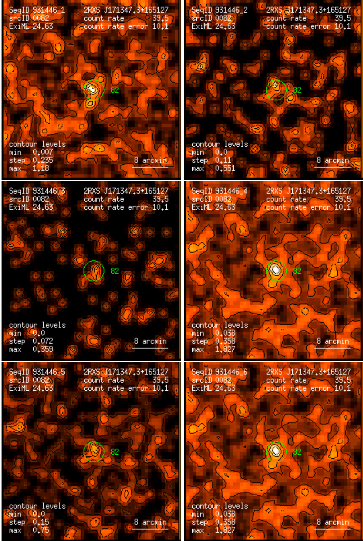
Figure 82: RASS 931446: detection 0082: band rate images, Gaussian filter: (1) PSPC channels 11 – 41, (2) 52 – 90, (3) 91 – 201, (4) 11 – 235, (5) 52 – 201, (6) 11 – 201. Broad band rates in counts/ks. Band rate contour levels in counts/ks/arcmin 2 .
