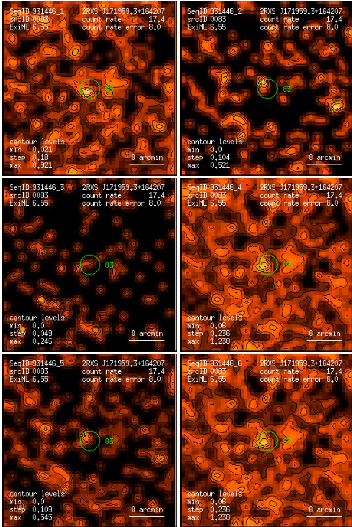
Figure 83: RASS 931446: detection 0083: band rate images, Gaussian filter: (1) PSPC channels 11 – 41, (2) 52 – 90, (3) 91 – 201, (4) 11 – 235, (5) 52 – 201, (6) 11 – 201. Broad band rates in counts/ks. Band rate contour levels in counts/ks/arcmin 2 .
