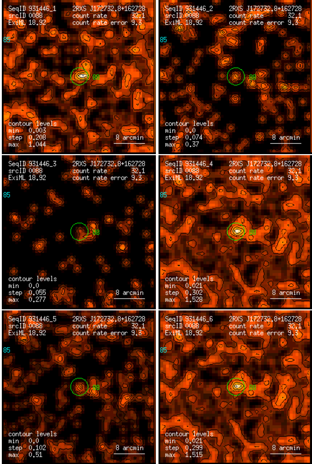
Figure 88: RASS 931446: detection 0088: band rate images, Gaussian filter: (1) PSPC channels 11 – 41, (2) 52 – 90, (3) 91 – 201, (4) 11 – 235, (5) 52 – 201, (6) 11 – 201. Broad band rates in counts/ks. Band rate contour levels in counts/ks/arcmin 2 .
