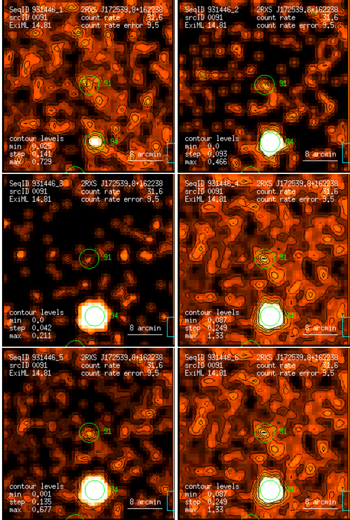
Figure 91: RASS 931446: detection 0091: band rate images, Gaussian filter: (1) PSPC channels 11 – 41, (2) 52 – 90, (3) 91 – 201, (4) 11 – 235, (5) 52 – 201, (6) 11 – 201. Broad band rates in counts/ks. Band rate contour levels in counts/ks/arcmin 2 .
