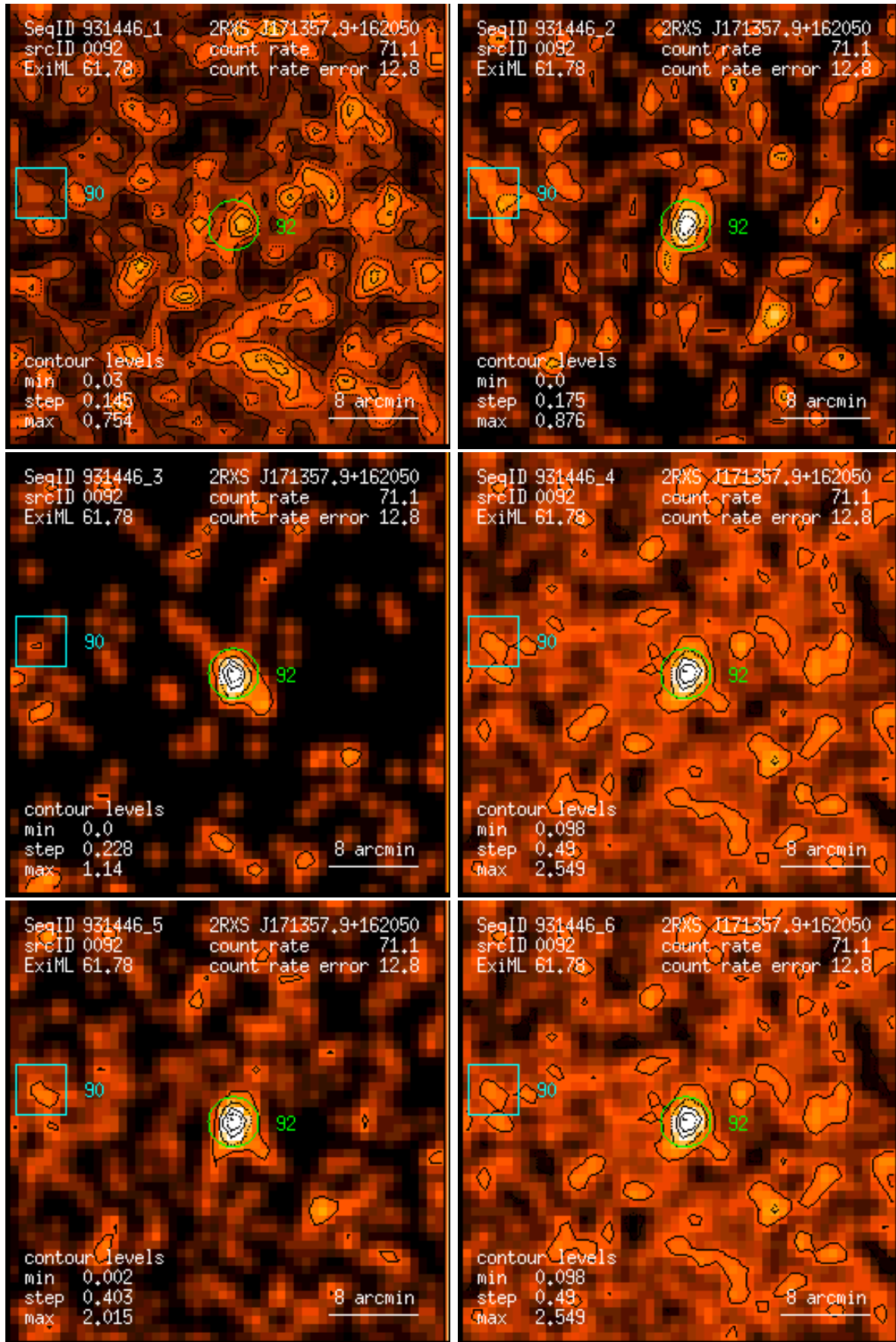
Figure 92: RASS 931446: detection 0092: band rate images, Gaussian filter: (1) PSPC channels 11 – 41, (2) 52 – 90, (3) 91 – 201, (4) 11 – 235, (5) 52 – 201, (6) 11 – 201. Broad band rates in counts/ks. Band rate contour levels in counts/ks/arcmin 2 .
