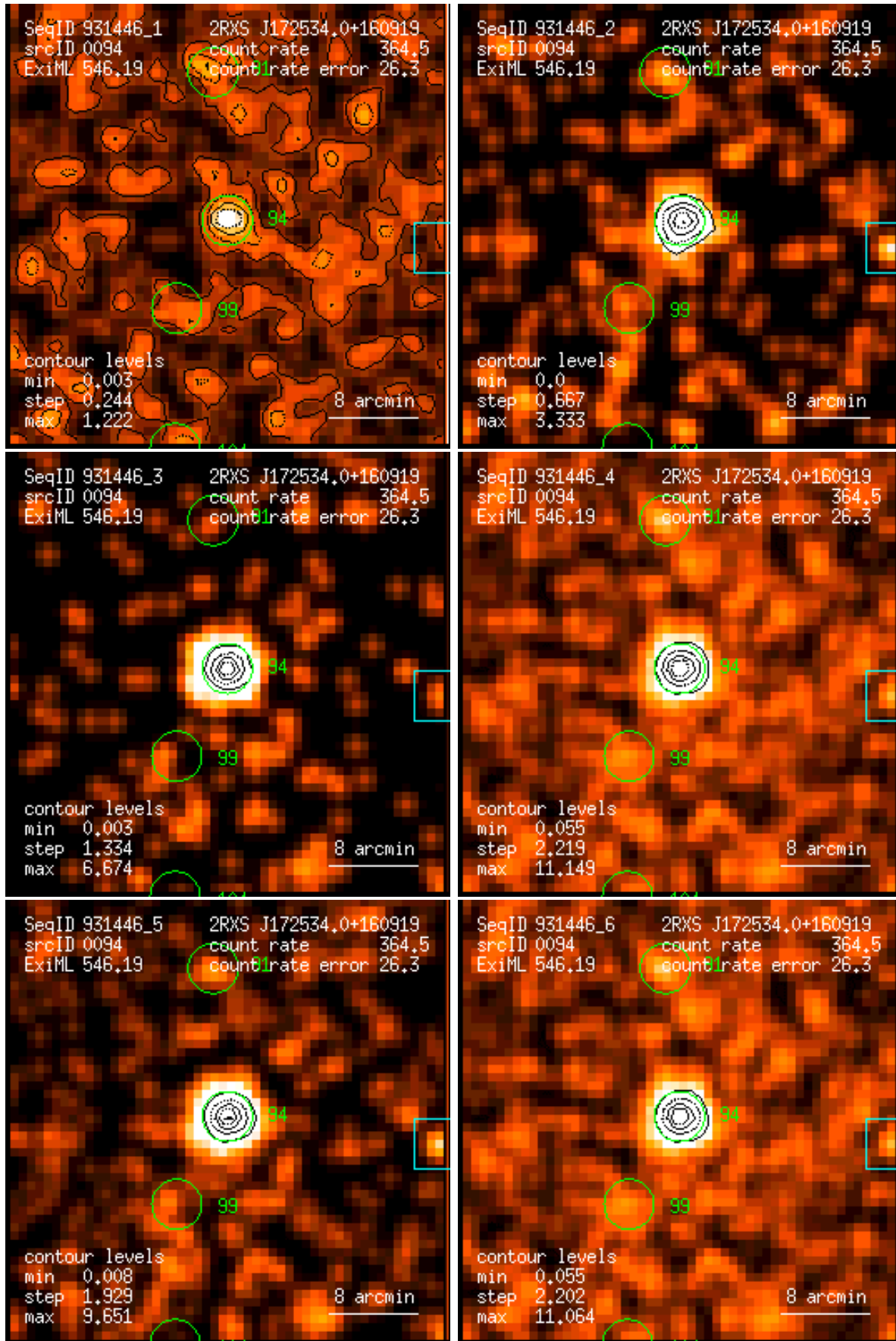
Figure 94: RASS 931446: detection 0094: band rate images, Gaussian filter: (1) PSPC channels 11 – 41, (2) 52 – 90, (3) 91 – 201, (4) 11 – 235, (5) 52 – 201, (6) 11 – 201. Broad band rates in counts/ks. Band rate contour levels in counts/ks/arcmin 2 .
