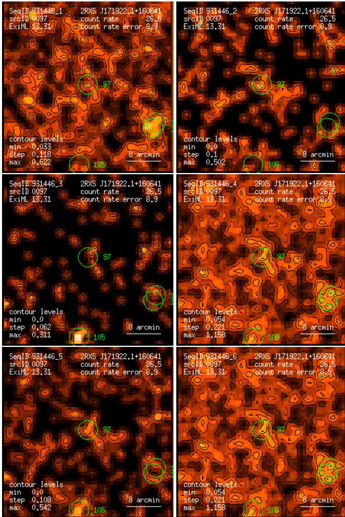
Figure 97: RASS 931446: detection 0097: band rate images, Gaussian filter: (1) PSPC channels 11 – 41, (2) 52 – 90, (3) 91 – 201, (4) 11 – 235, (5) 52 – 201, (6) 11 – 201. Broad band rates in counts/ks. Band rate contour levels in counts/ks/arcmin 2 .
