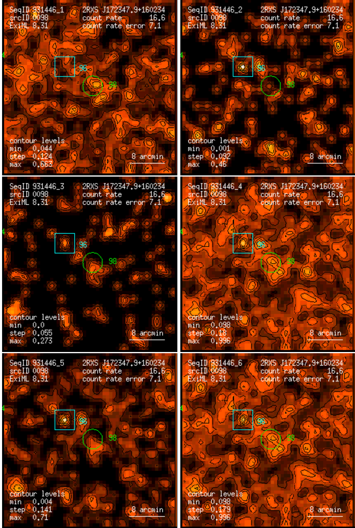
Figure 98: RASS 931446: detection 0098: band rate images, Gaussian filter: (1) PSPC channels 11 – 41, (2) 52 – 90, (3) 91 – 201, (4) 11 – 235, (5) 52 – 201, (6) 11 – 201. Broad band rates in counts/ks. Band rate contour levels in counts/ks/arcmin 2 .
