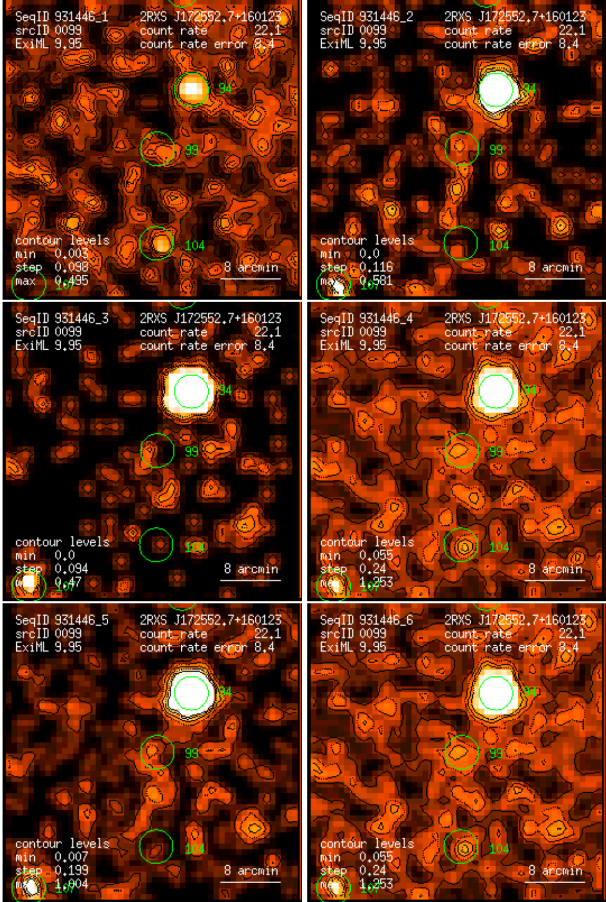
Figure 99: RASS 931446: detection 0099: band rate images, Gaussian filter: (1) PSPC channels 11 – 41, (2) 52 – 90, (3) 91 – 201, (4) 11 – 235, (5) 52 – 201, (6) 11 – 201. Broad band rates in counts/ks. Band rate contour levels in counts/ks/arcmin 2 .
