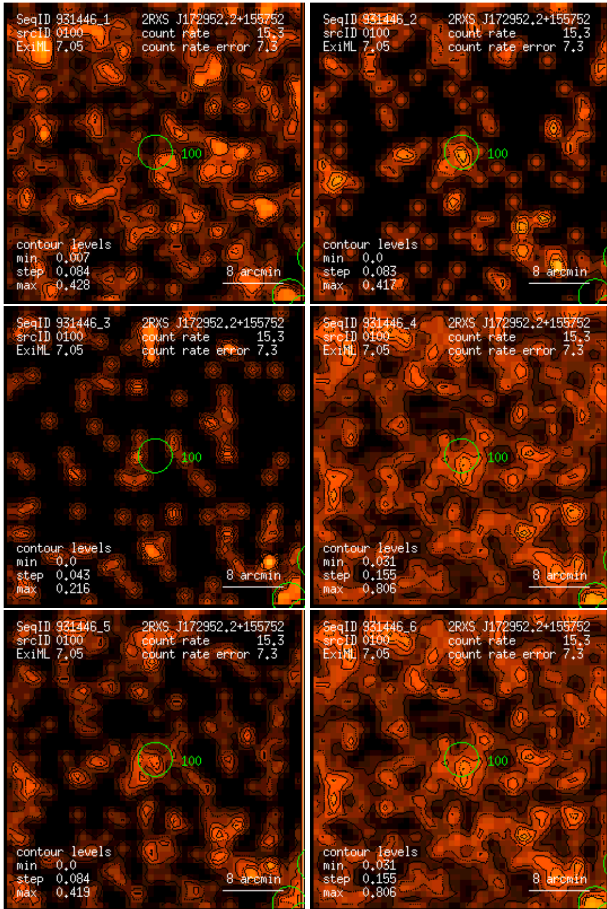
Figure 100: RASS 931446: detection 0100: band rate images, Gaussian filter: (1) PSPC channels 11 – 41, (2) 52 – 90, (3) 91 – 201, (4) 11 – 235, (5) 52 – 201, (6) 11 – 201. Broad band rates in counts/ks. Band rate contour levels in counts/ks/arcmin 2 .
