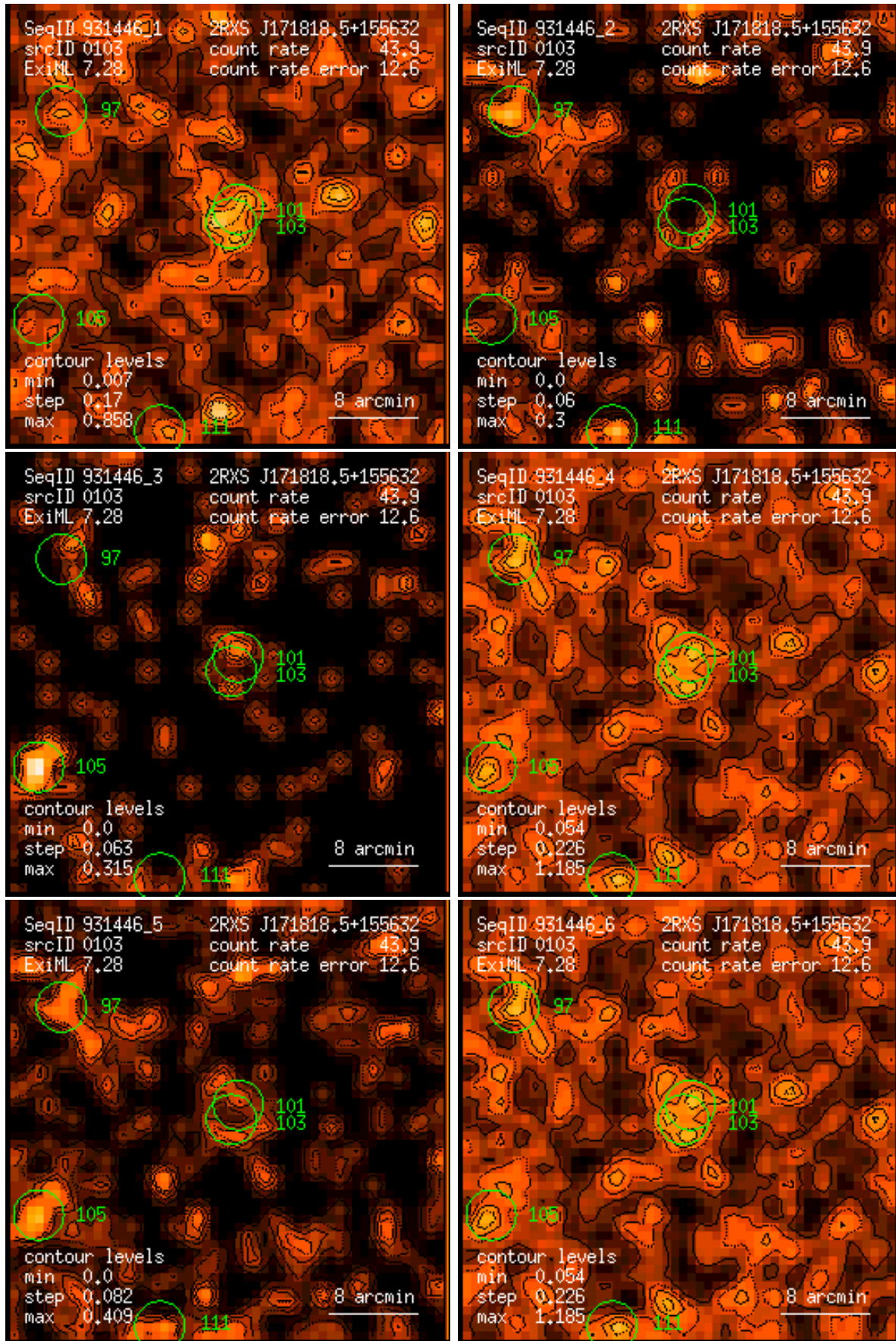
Figure 103: RASS 931446: detection 0103: band rate images, Gaussian filter: (1) PSPC channels 11 – 41, (2) 52 – 90, (3) 91 – 201, (4) 11 – 235, (5) 52 – 201, (6) 11 – 201. Broad band rates in counts/ks. Band rate contour levels in counts/ks/arcmin 2 .
