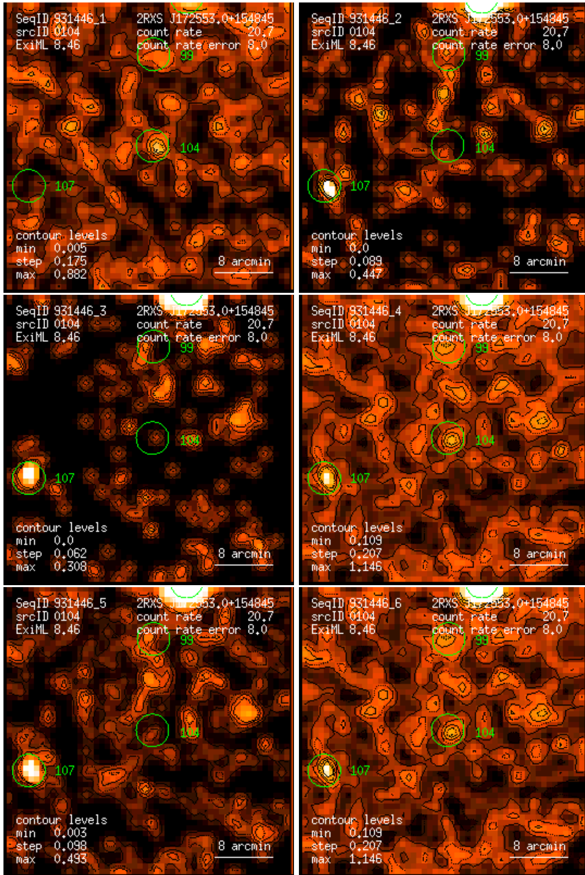
Figure 104: RASS 931446: detection 0104: band rate images, Gaussian filter: (1) PSPC channels 11 – 41, (2) 52 – 90, (3) 91 – 201, (4) 11 – 235, (5) 52 – 201, (6) 11 – 201. Broad band rates in counts/ks. Band rate contour levels in counts/ks/arcmin 2 .
