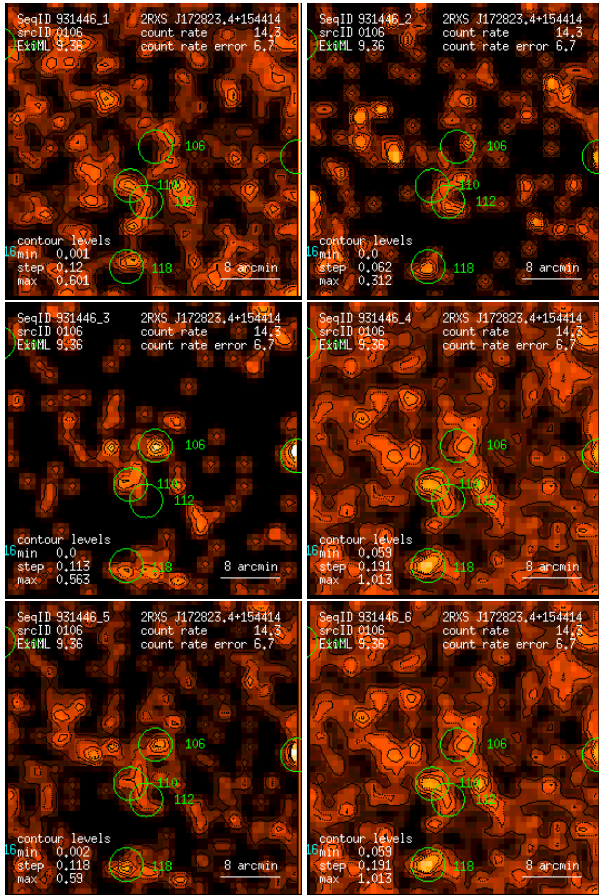
Figure 106: RASS 931446: detection 0106: band rate images, Gaussian filter: (1) PSPC channels 11 – 41, (2) 52 – 90, (3) 91 – 201, (4) 11 – 235, (5) 52 – 201, (6) 11 – 201. Broad band rates in counts/ks. Band rate contour levels in counts/ks/arcmin 2 .
