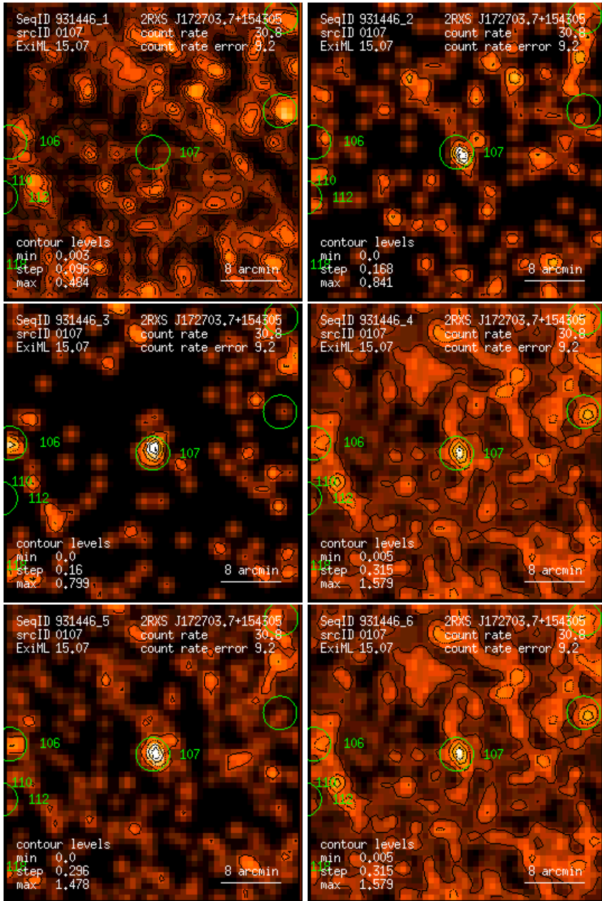
Figure 107: RASS 931446: detection 0107: band rate images, Gaussian filter: (1) PSPC channels 11 – 41, (2) 52 – 90, (3) 91 – 201, (4) 11 – 235, (5) 52 – 201, (6) 11 – 201. Broad band rates in counts/ks. Band rate contour levels in counts/ks/arcmin 2 .
