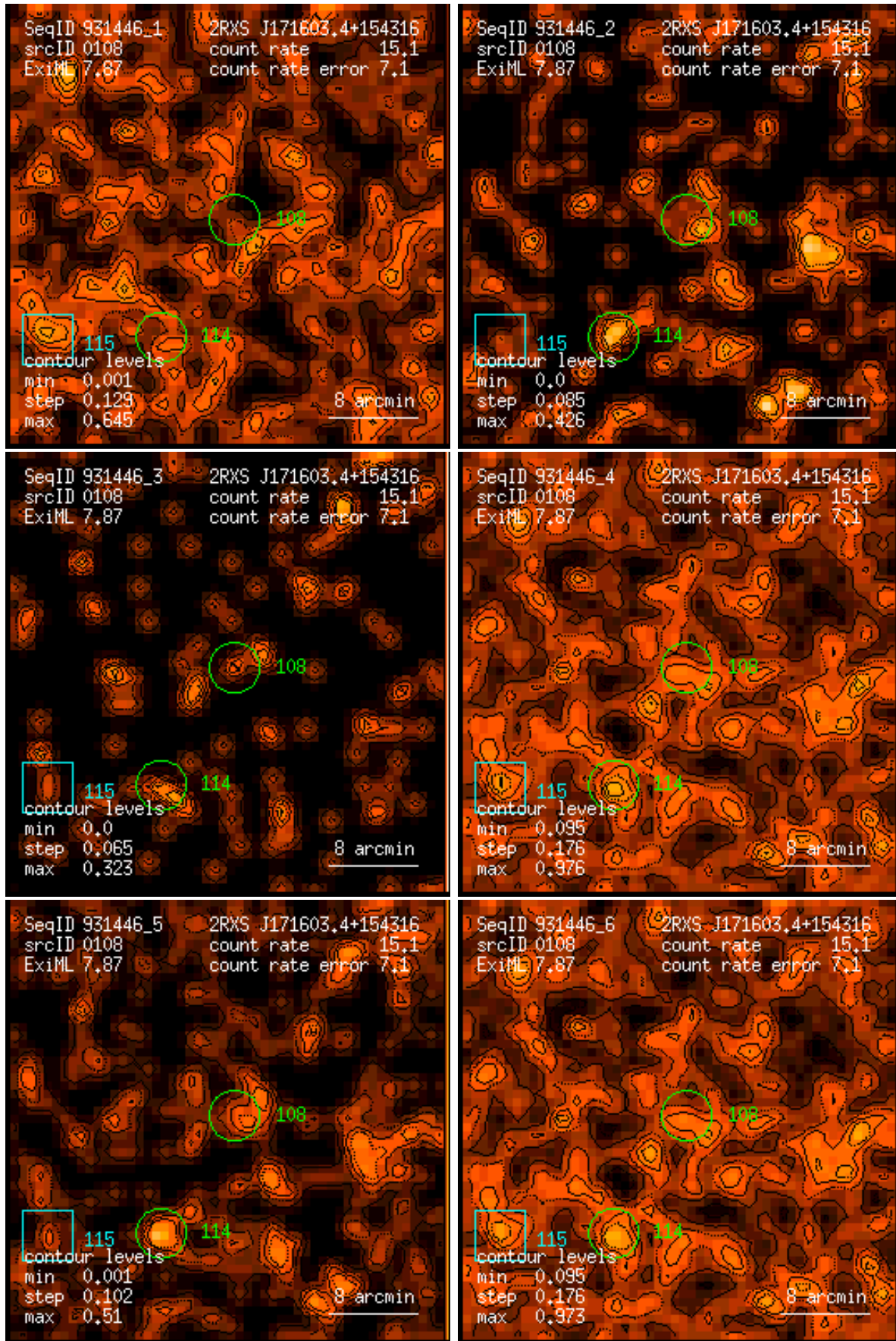
Figure 108: RASS 931446: detection 0108: band rate images, Gaussian filter: (1) PSPC channels 11 – 41, (2) 52 – 90, (3) 91 – 201, (4) 11 – 235, (5) 52 – 201, (6) 11 – 201. Broad band rates in counts/ks. Band rate contour levels in counts/ks/arcmin 2 .
