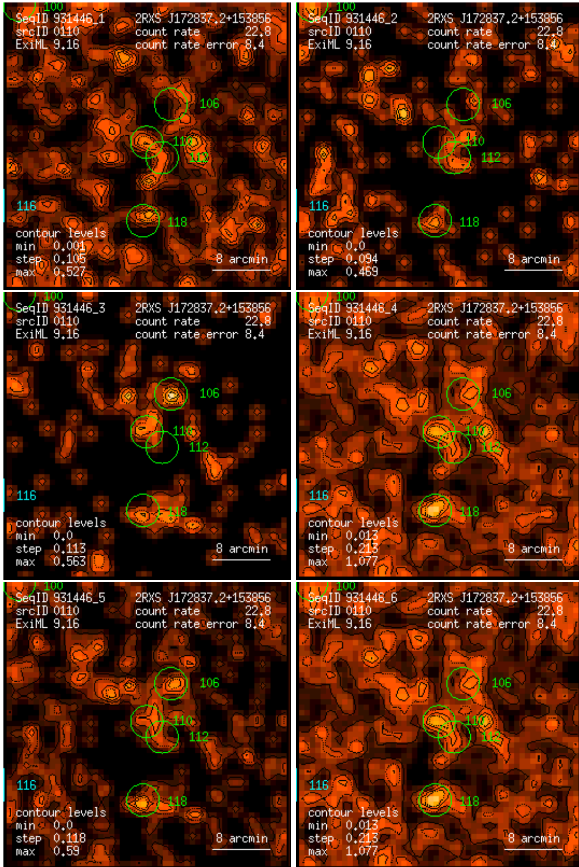
Figure 110: RASS 931446: detection 0110: band rate images, Gaussian filter: (1) PSPC channels 11 – 41, (2) 52 – 90, (3) 91 – 201, (4) 11 – 235, (5) 52 – 201, (6) 11 – 201. Broad band rates in counts/ks. Band rate contour levels in counts/ks/arcmin 2 .
