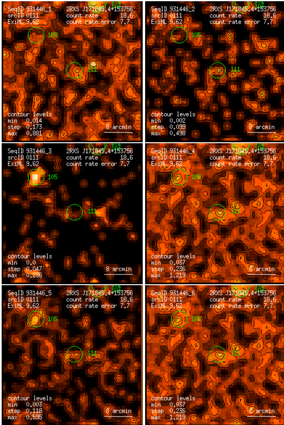
Figure 111: RASS 931446: detection 0111: band rate images, Gaussian filter: (1) PSPC channels 11 – 41, (2) 52 – 90, (3) 91 – 201, (4) 11 – 235, (5) 52 – 201, (6) 11 – 201. Broad band rates in counts/ks. Band rate contour levels in counts/ks/arcmin 2 .
