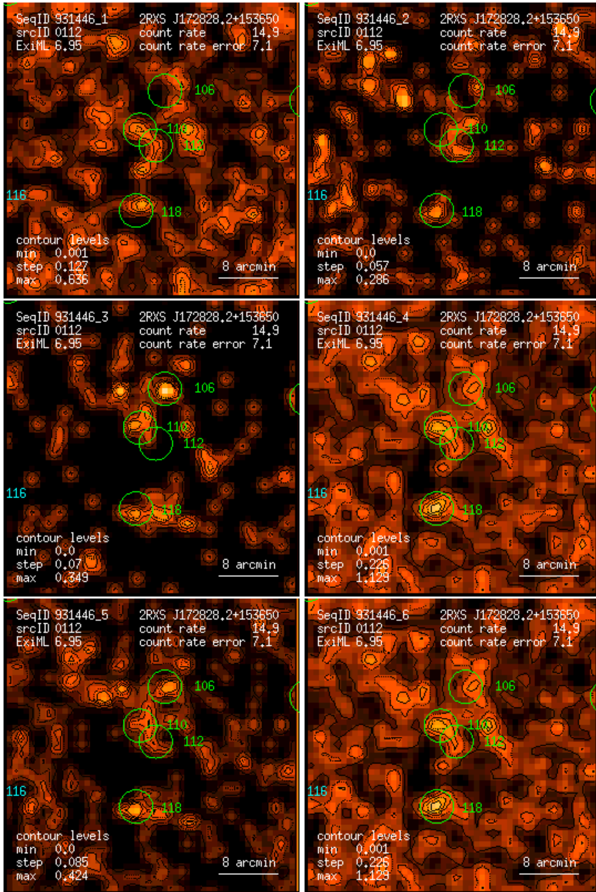
Figure 112: RASS 931446: detection 0112: band rate images, Gaussian filter: (1) PSPC channels 11 – 41, (2) 52 – 90, (3) 91 – 201, (4) 11 – 235, (5) 52 – 201, (6) 11 – 201. Broad band rates in counts/ks. Band rate contour levels in counts/ks/arcmin 2 .
