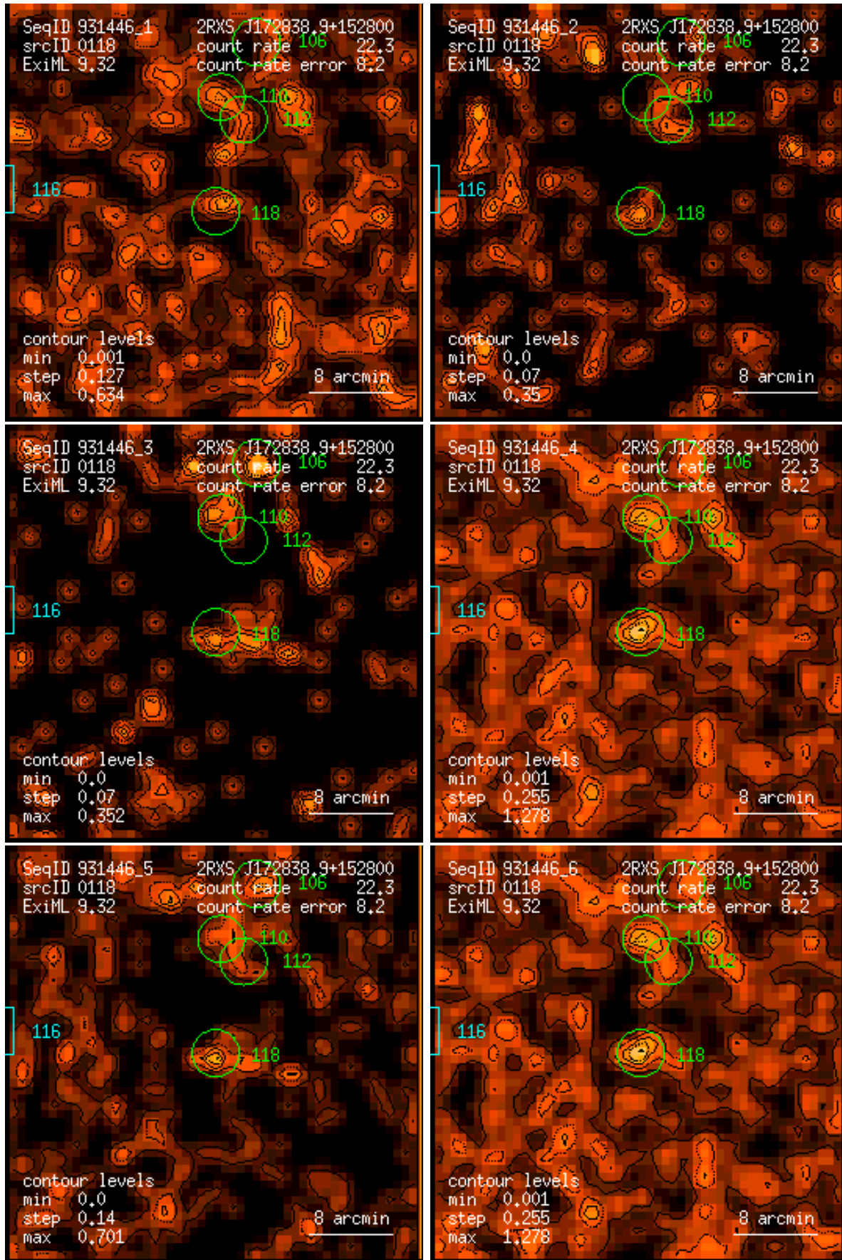
Figure 118: RASS 931446: detection 0118: band rate images, Gaussian filter: (1) PSPC channels 11 – 41, (2) 52 – 90, (3) 91 – 201, (4) 11 – 235, (5) 52 – 201, (6) 11 – 201. Broad band rates in counts/ks. Band rate contour levels in counts/ks/arcmin 2 .
