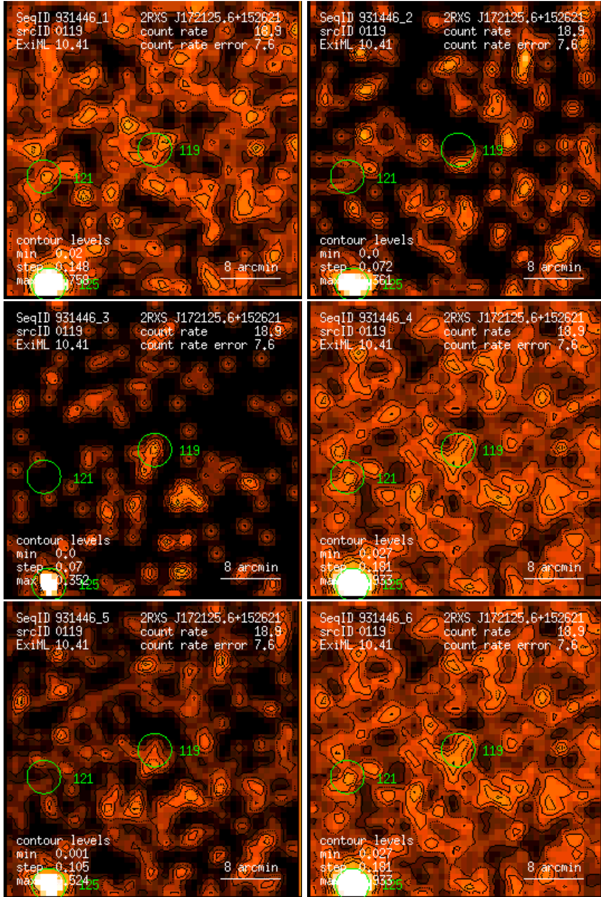
Figure 119: RASS 931446: detection 0119: band rate images, Gaussian filter: (1) PSPC channels 11 – 41, (2) 52 – 90, (3) 91 – 201, (4) 11 – 235, (5) 52 – 201, (6) 11 – 201. Broad band rates in counts/ks. Band rate contour levels in counts/ks/arcmin 2 .
