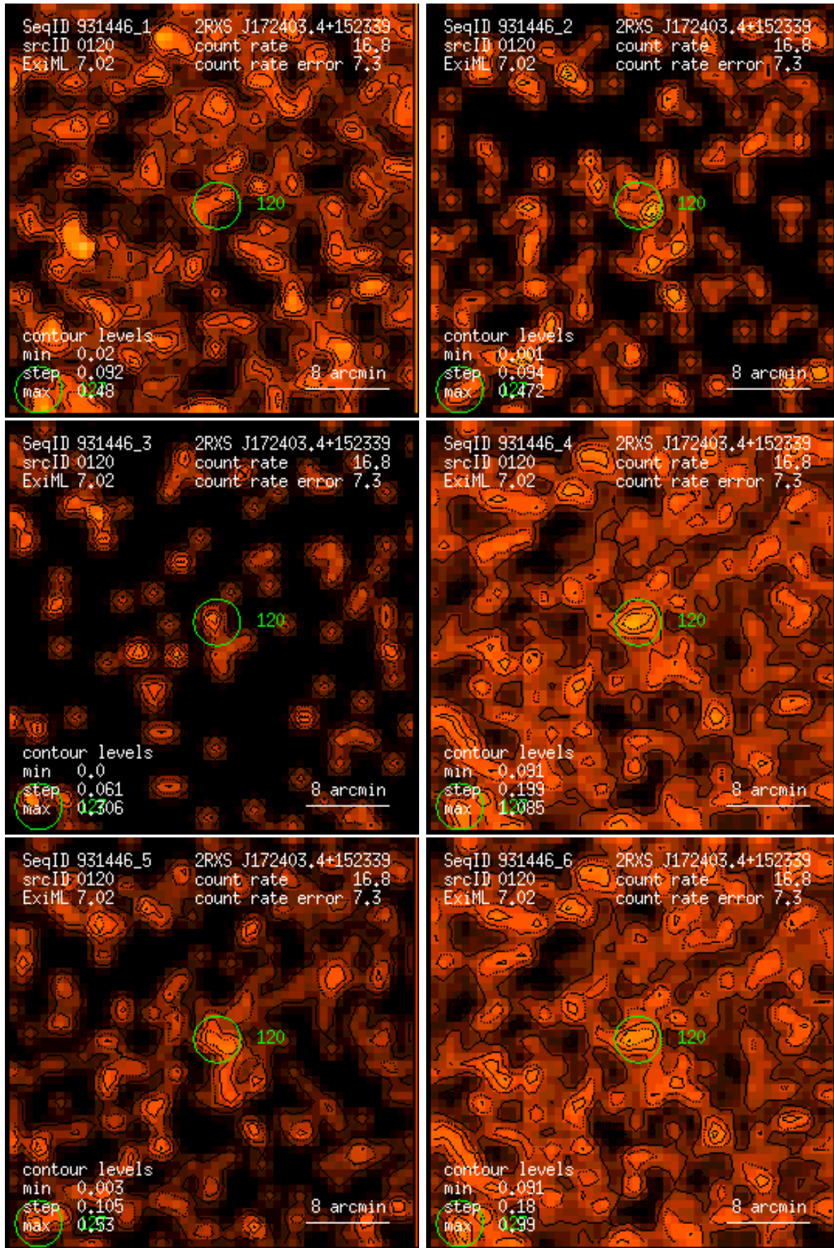
Figure 120: RASS 931446: detection 0120: band rate images, Gaussian filter: (1) PSPC channels 11 – 41, (2) 52 – 90, (3) 91 – 201, (4) 11 – 235, (5) 52 – 201, (6) 11 – 201. Broad band rates in counts/ks. Band rate contour levels in counts/ks/arcmin 2 .
