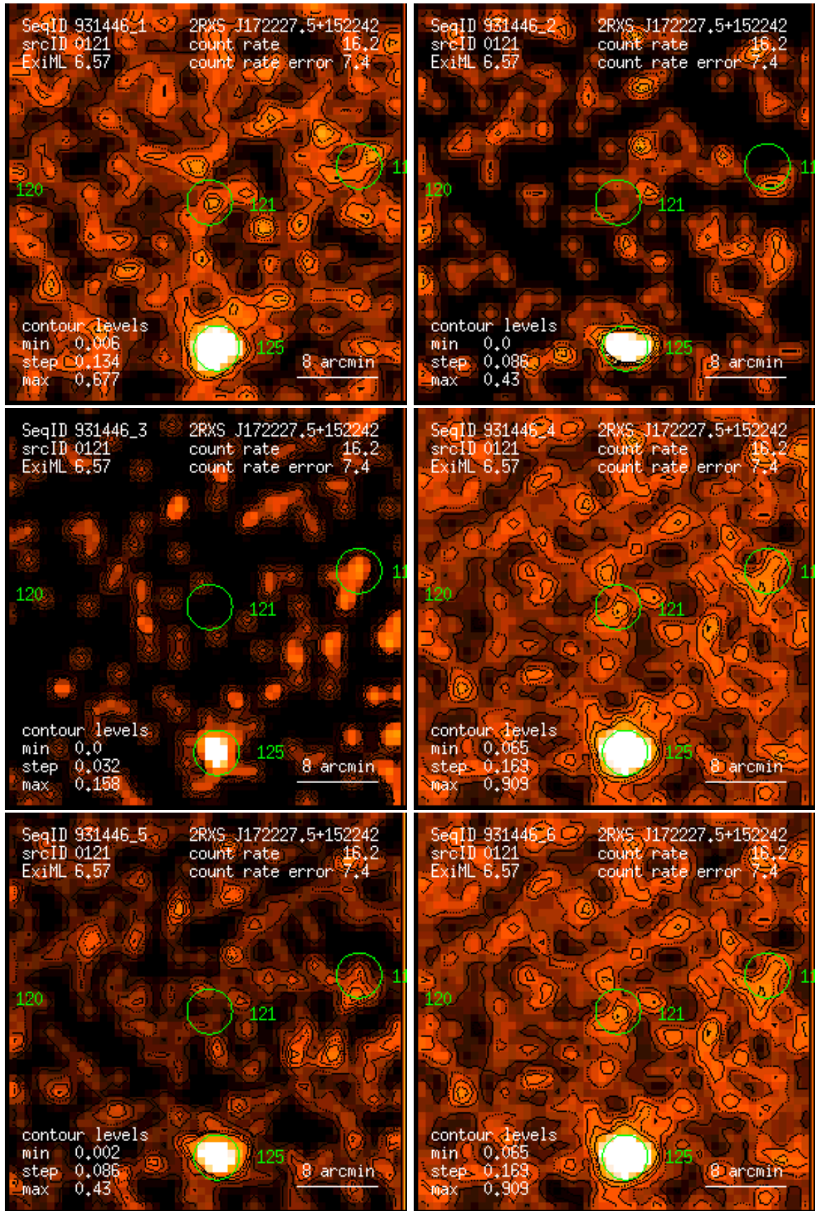
Figure 121: RASS 931446: detection 0121: band rate images, Gaussian filter: (1) PSPC channels 11 – 41, (2) 52 – 90, (3) 91 – 201, (4) 11 – 235, (5) 52 – 201, (6) 11 – 201. Broad band rates in counts/ks. Band rate contour levels in counts/ks/arcmin 2 .
