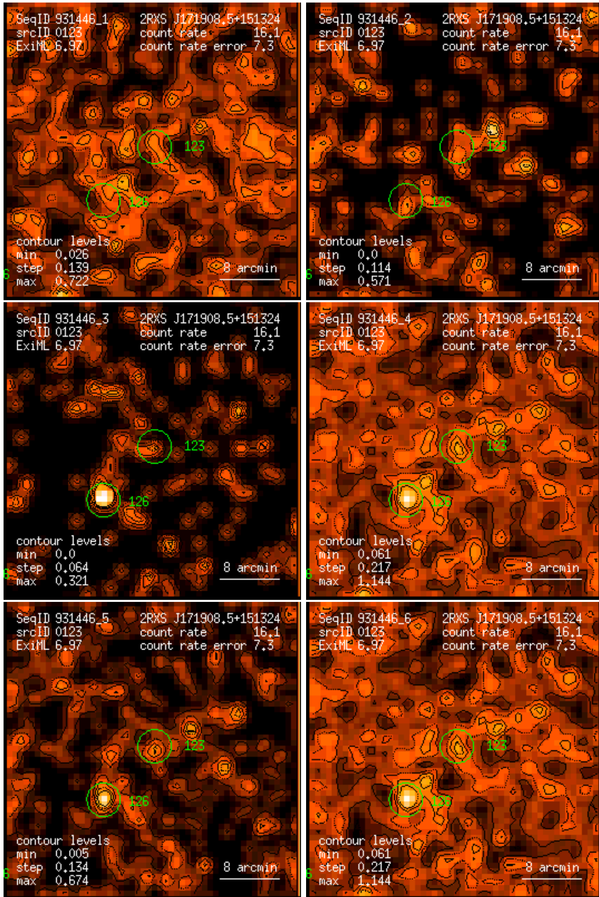
Figure 123: RASS 931446: detection 0123: band rate images, Gaussian filter: (1) PSPC channels 11 – 41, (2) 52 – 90, (3) 91 – 201, (4) 11 – 235, (5) 52 – 201, (6) 11 – 201. Broad band rates in counts/ks. Band rate contour levels in counts/ks/arcmin 2 .
