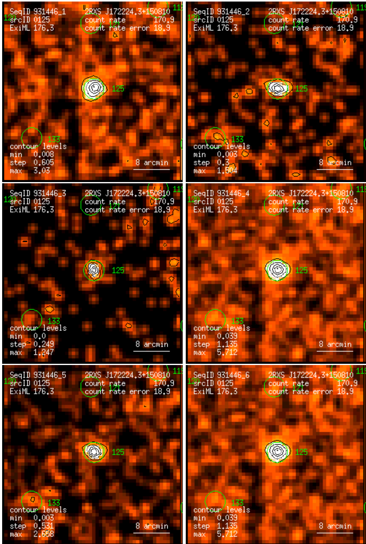
Figure 125: RASS 931446: detection 0125: band rate images, Gaussian filter: (1) PSPC channels 11 – 41, (2) 52 – 90, (3) 91 – 201, (4) 11 – 235, (5) 52 – 201, (6) 11 – 201. Broad band rates in counts/ks. Band rate contour levels in counts/ks/arcmin 2 .
