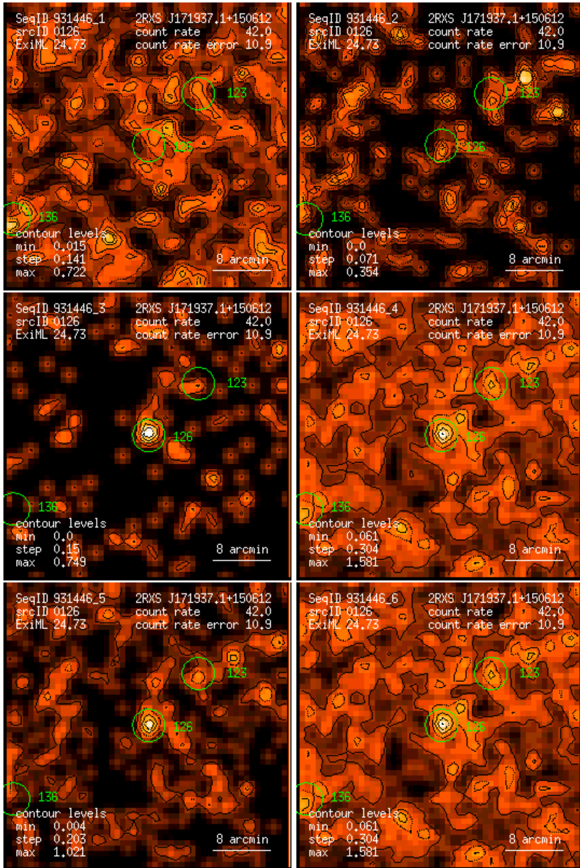
Figure 126: RASS 931446: detection 0126: band rate images, Gaussian filter: (1) PSPC channels 11 – 41, (2) 52 – 90, (3) 91 – 201, (4) 11 – 235, (5) 52 – 201, (6) 11 – 201. Broad band rates in counts/ks. Band rate contour levels in counts/ks/arcmin 2 .
