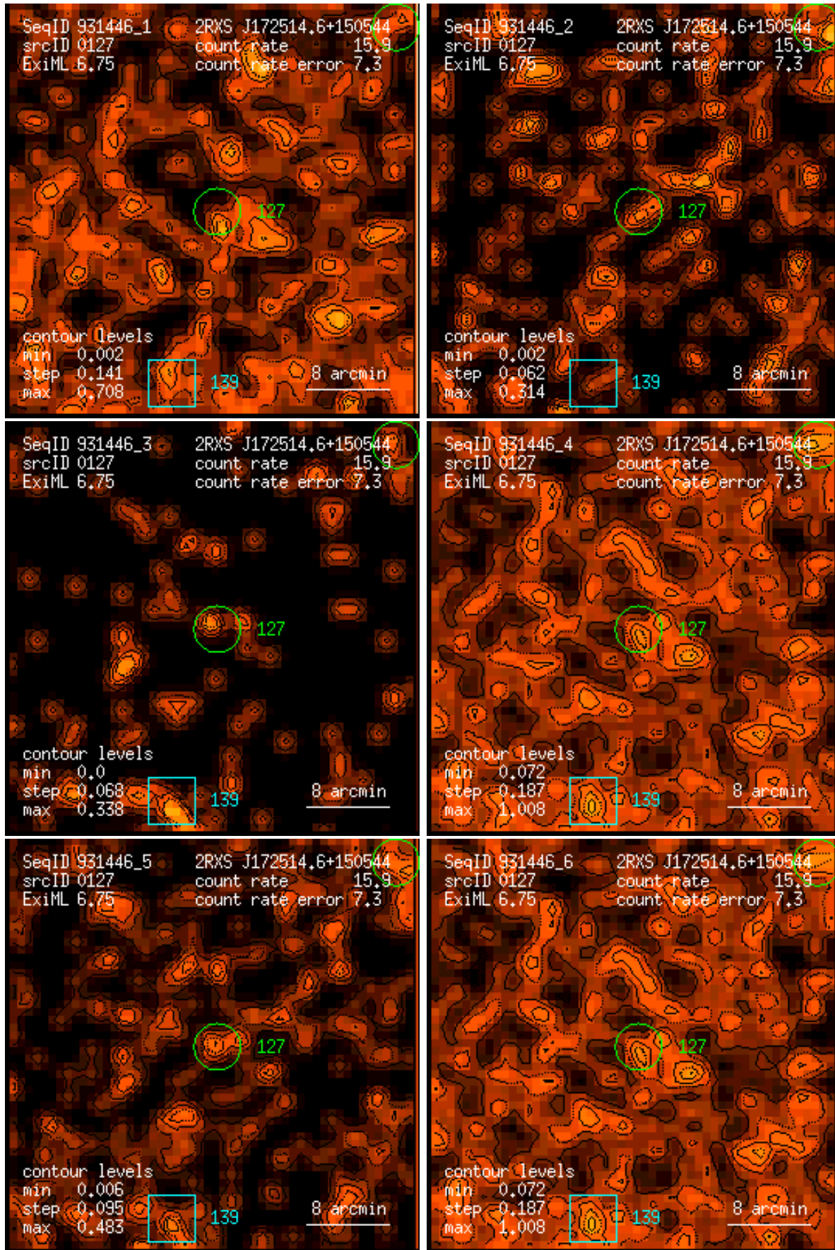
Figure 127: RASS 931446: detection 0127: band rate images, Gaussian filter: (1) PSPC channels 11 – 41, (2) 52 – 90, (3) 91 – 201, (4) 11 – 235, (5) 52 – 201, (6) 11 – 201. Broad band rates in counts/ks. Band rate contour levels in counts/ks/arcmin 2 .
