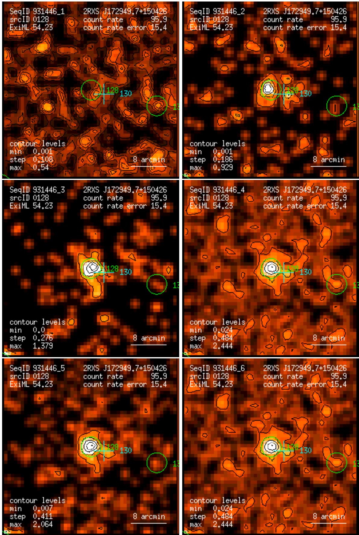
Figure 128: RASS 931446: detection 0128: band rate images, Gaussian filter: (1) PSPC channels 11 – 41, (2) 52 – 90, (3) 91 – 201, (4) 11 – 235, (5) 52 – 201, (6) 11 – 201. Broad band rates in counts/ks. Band rate contour levels in counts/ks/arcmin 2 .
