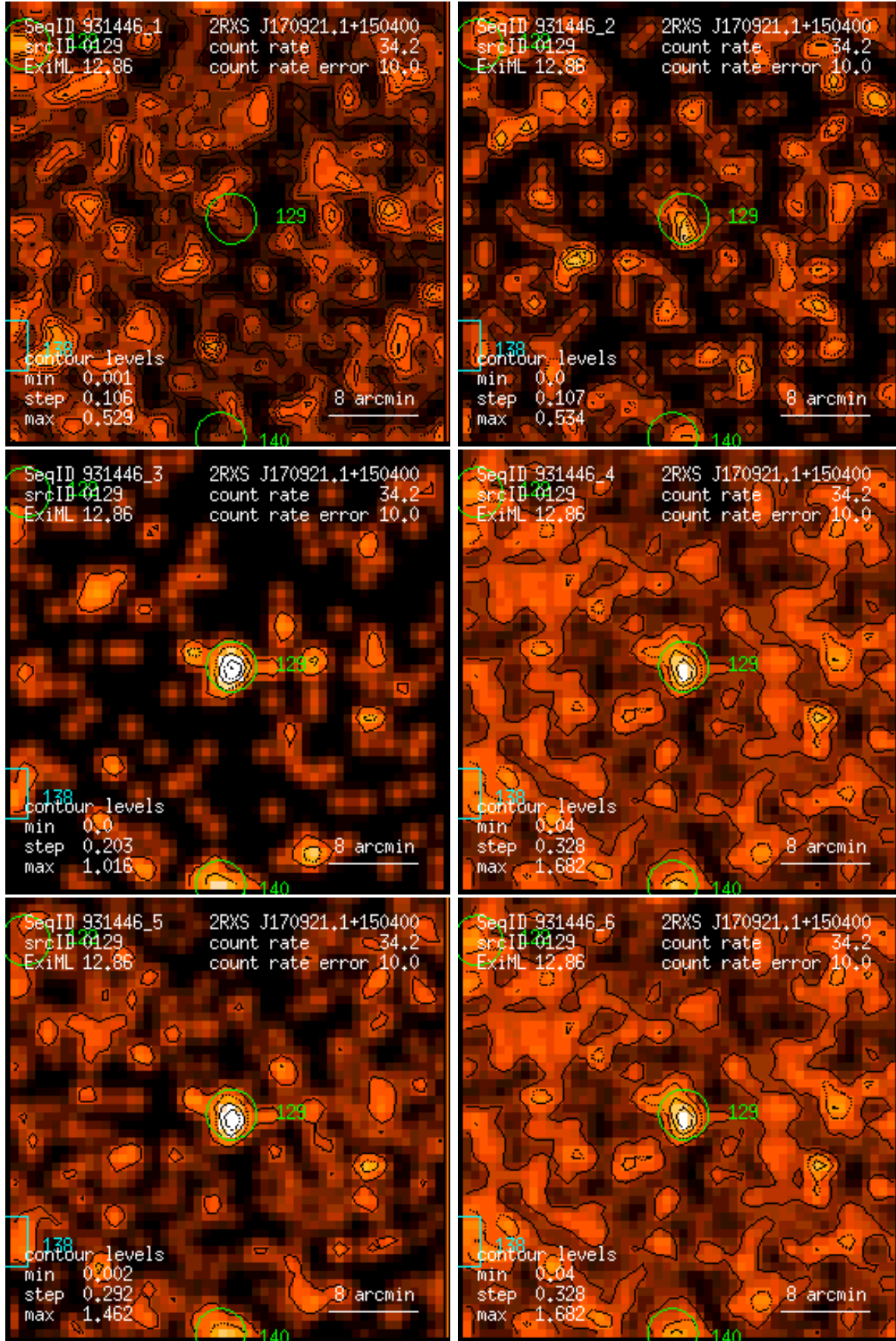
Figure 129: RASS 931446: detection 0129: band rate images, Gaussian filter: (1) PSPC channels 11 – 41, (2) 52 – 90, (3) 91 – 201, (4) 11 – 235, (5) 52 – 201, (6) 11 – 201. Broad band rates in counts/ks. Band rate contour levels in counts/ks/arcmin 2 .
