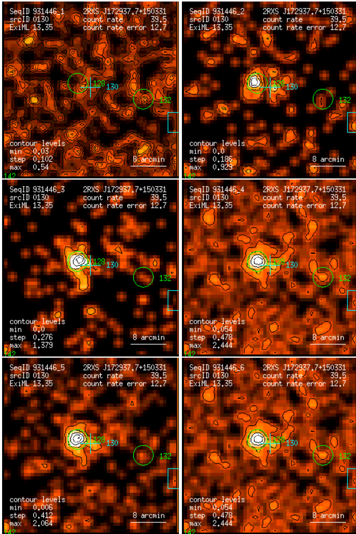
Figure 130: RASS 931446: detection 0130: band rate images, Gaussian filter: (1) PSPC channels 11 – 41, (2) 52 – 90, (3) 91 – 201, (4) 11 – 235, (5) 52 – 201, (6) 11 – 201. Broad band rates in counts/ks. Band rate contour levels in counts/ks/arcmin 2 .
