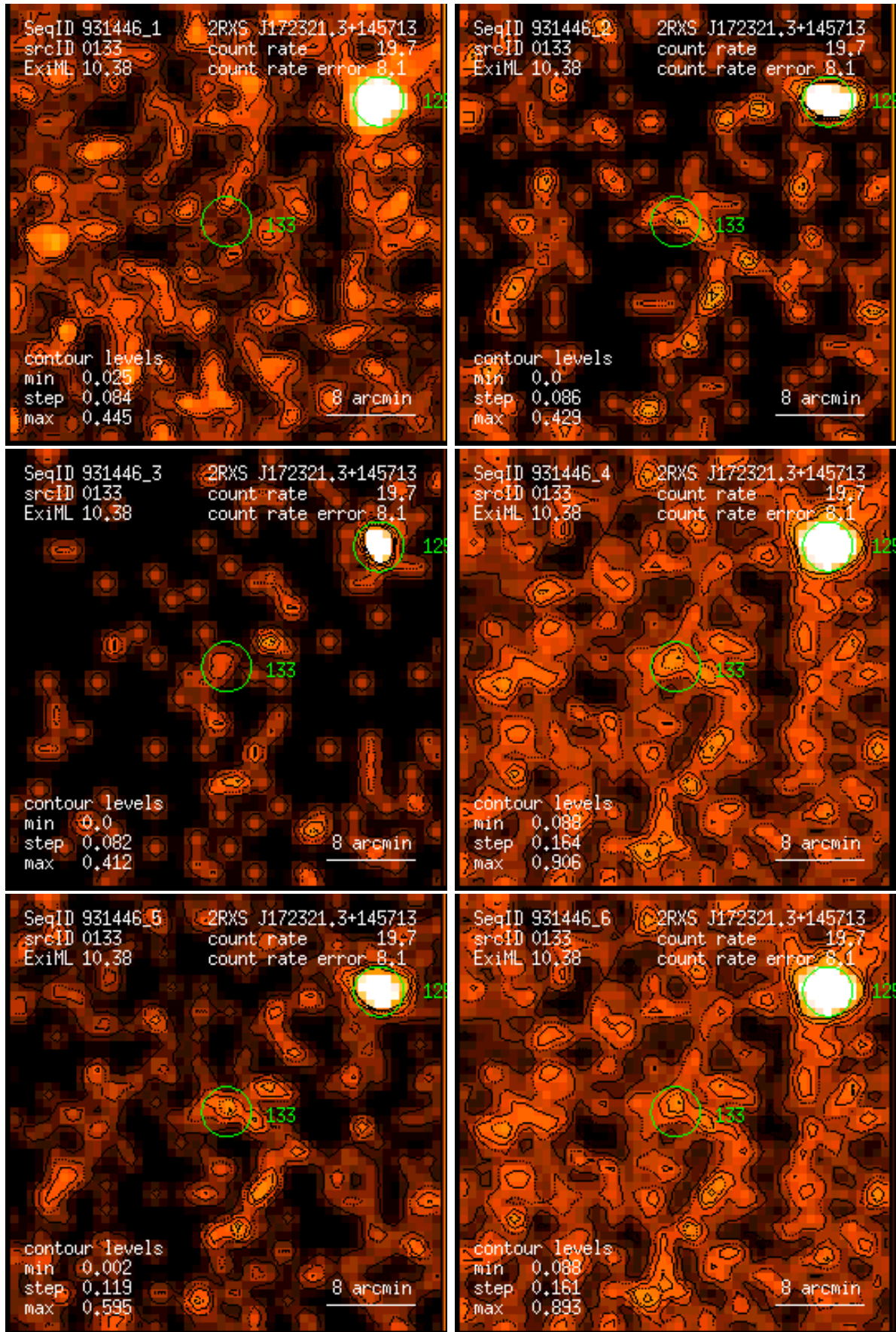
Figure 133: RASS 931446: detection 0133: band rate images, Gaussian filter: (1) PSPC channels 11 – 41, (2) 52 – 90, (3) 91 – 201, (4) 11 – 235, (5) 52 – 201, (6) 11 – 201. Broad band rates in counts/ks. Band rate contour levels in counts/ks/arcmin 2 .
