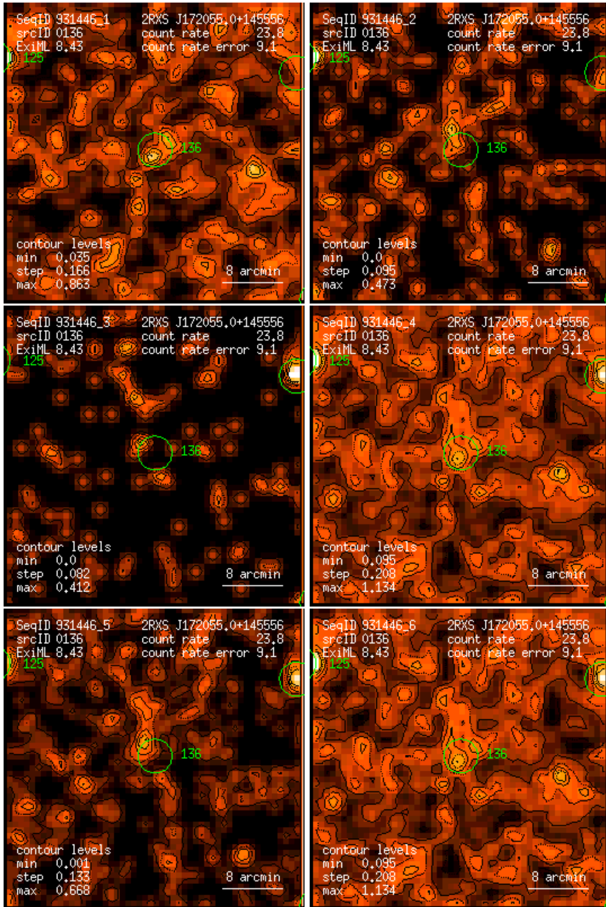
Figure 136: RASS 931446: detection 0136: band rate images, Gaussian filter: (1) PSPC channels 11 – 41, (2) 52 – 90, (3) 91 – 201, (4) 11 – 235, (5) 52 – 201, (6) 11 – 201. Broad band rates in counts/ks. Band rate contour levels in counts/ks/arcmin 2 .
