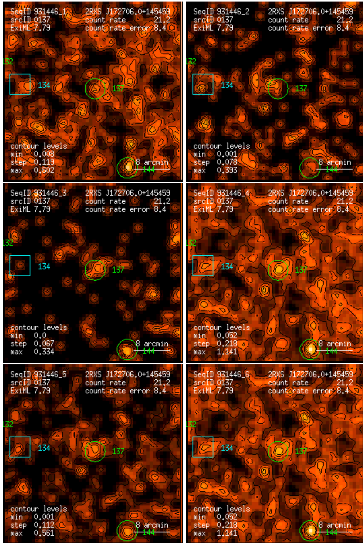
Figure 137: RASS 931446: detection 0137: band rate images, Gaussian filter: (1) PSPC channels 11 – 41, (2) 52 – 90, (3) 91 – 201, (4) 11 – 235, (5) 52 – 201, (6) 11 – 201. Broad band rates in counts/ks. Band rate contour levels in counts/ks/arcmin 2 .
