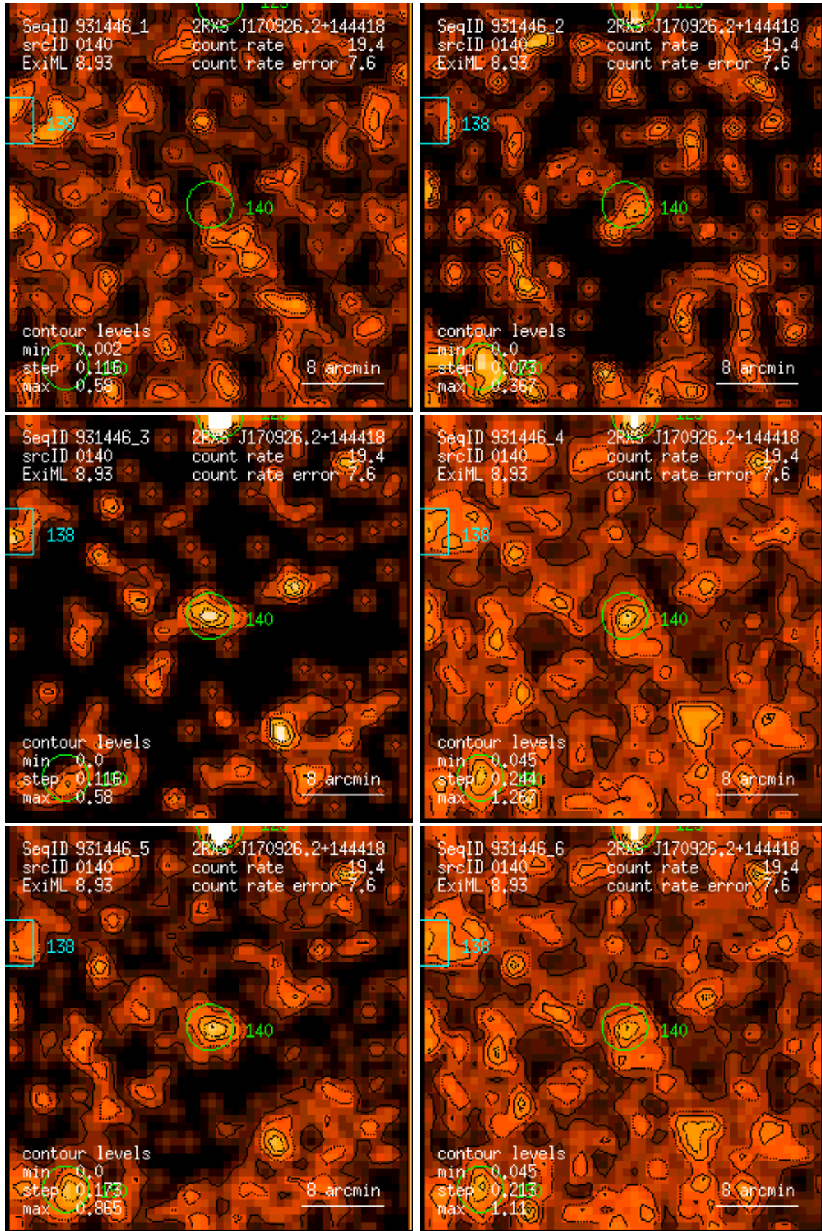
Figure 140: RASS 931446: detection 0140: band rate images, Gaussian filter: (1) PSPC channels 11 – 41, (2) 52 – 90, (3) 91 – 201, (4) 11 – 235, (5) 52 – 201, (6) 11 – 201. Broad band rates in counts/ks. Band rate contour levels in counts/ks/arcmin 2 .
