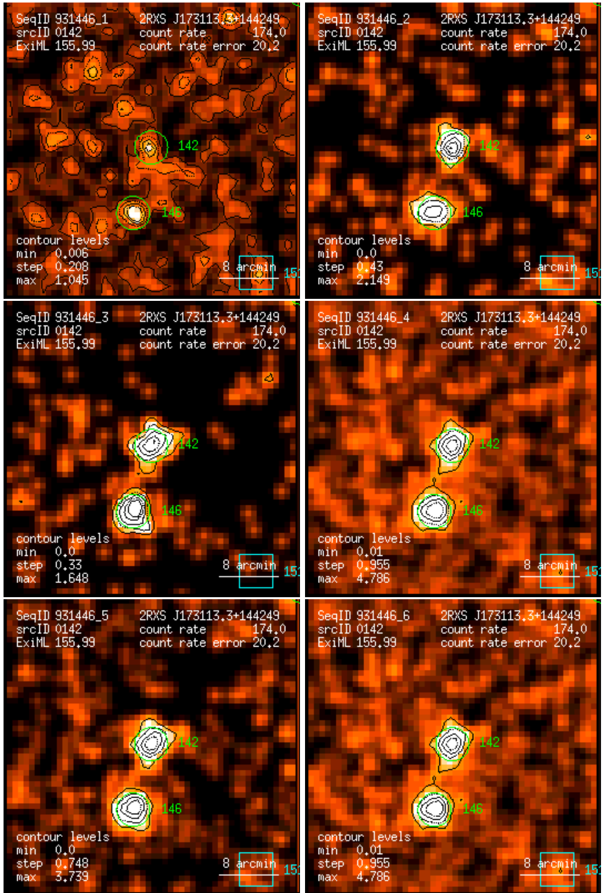
Figure 142: RASS 931446: detection 0142: band rate images, Gaussian filter: (1) PSPC channels 11 – 41, (2) 52 – 90, (3) 91 – 201, (4) 11 – 235, (5) 52 – 201, (6) 11 – 201. Broad band rates in counts/ks. Band rate contour levels in counts/ks/arcmin 2 .
