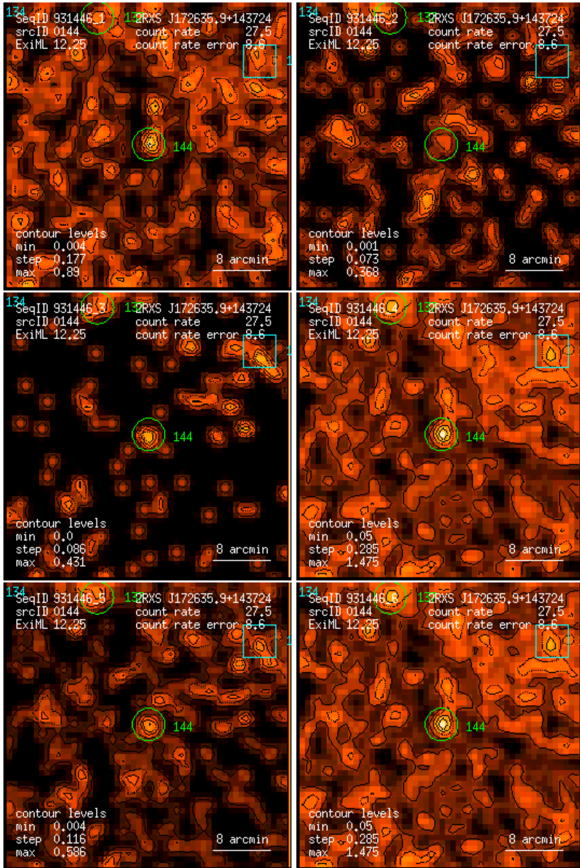
Figure 144: RASS 931446: detection 0144: band rate images, Gaussian filter: (1) PSPC channels 11 – 41, (2) 52 – 90, (3) 91 – 201, (4) 11 – 235, (5) 52 – 201, (6) 11 – 201. Broad band rates in counts/ks. Band rate contour levels in counts/ks/arcmin 2 .
