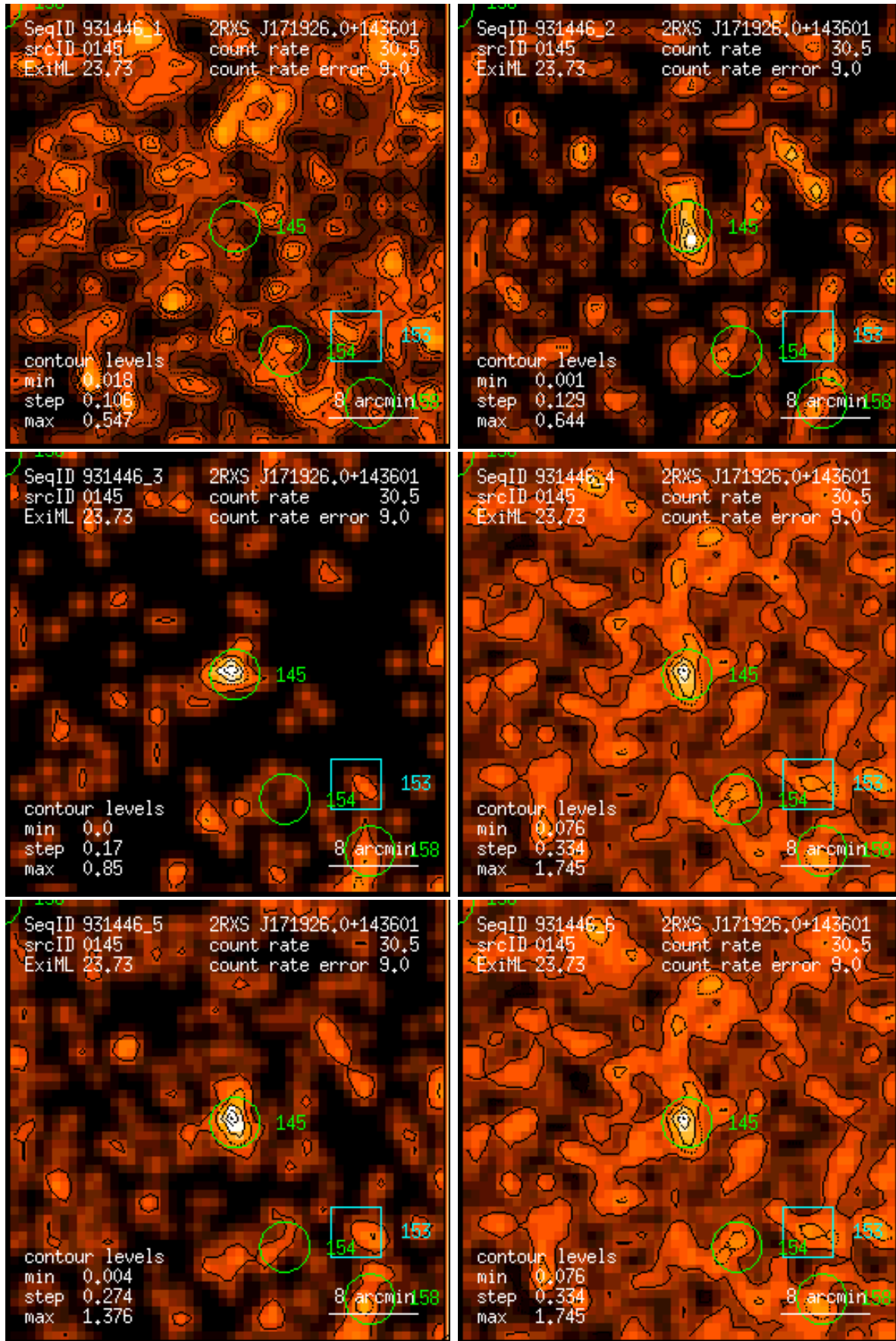
Figure 145: RASS 931446: detection 0145: band rate images, Gaussian filter: (1) PSPC channels 11 – 41, (2) 52 – 90, (3) 91 – 201, (4) 11 – 235, (5) 52 – 201, (6) 11 – 201. Broad band rates in counts/ks. Band rate contour levels in counts/ks/arcmin 2 .
