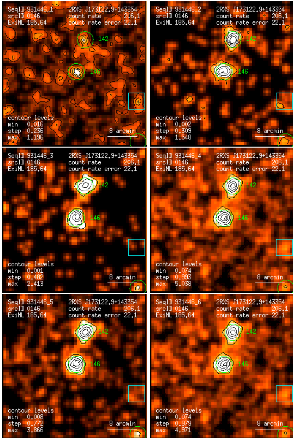
Figure 146: RASS 931446: detection 0146: band rate images, Gaussian filter: (1) PSPC channels 11 – 41, (2) 52 – 90, (3) 91 – 201, (4) 11 – 235, (5) 52 – 201, (6) 11 – 201. Broad band rates in counts/ks. Band rate contour levels in counts/ks/arcmin 2 .
