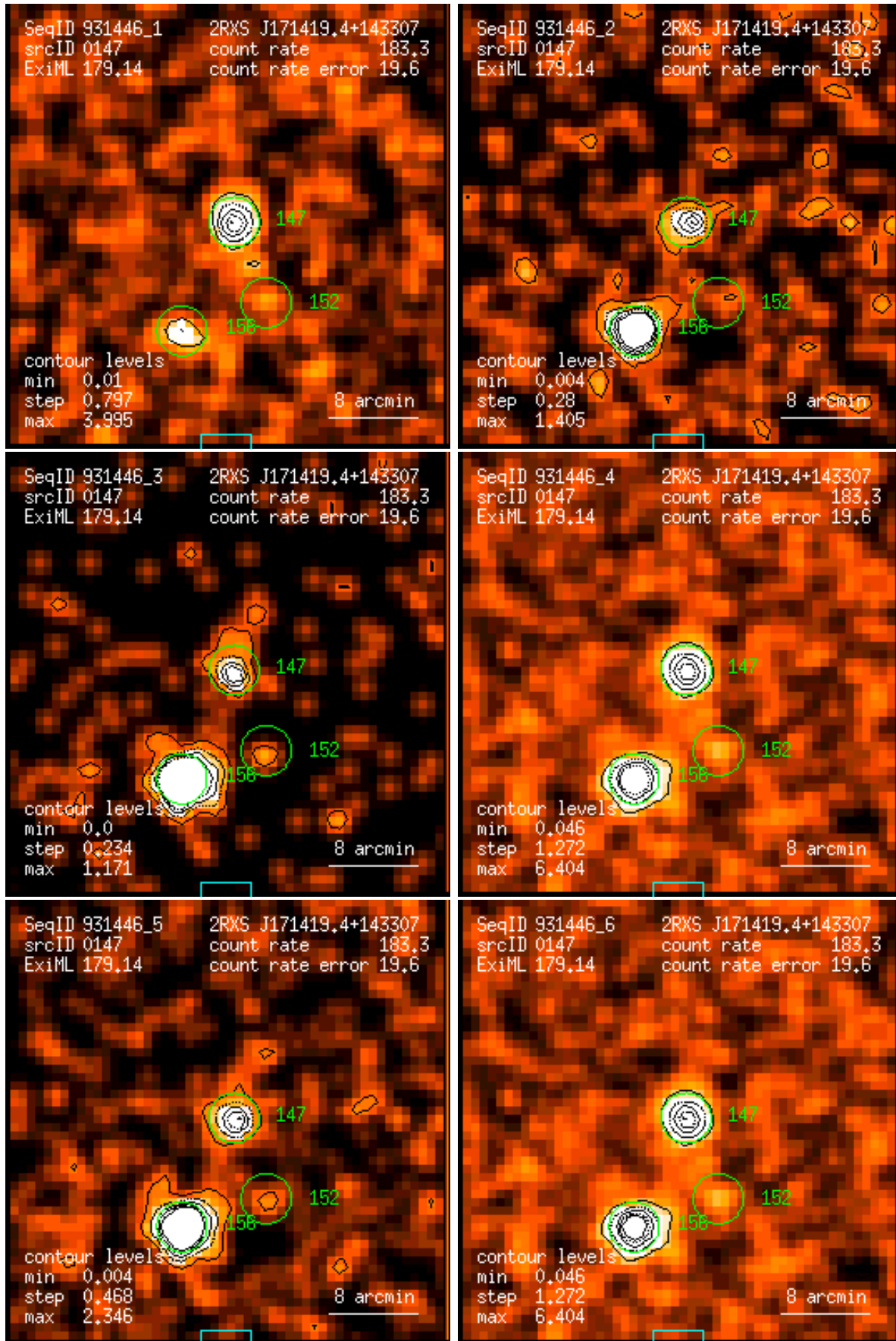
Figure 147: RASS 931446: detection 0147: band rate images, Gaussian filter: (1) PSPC channels 11 – 41, (2) 52 – 90, (3) 91 – 201, (4) 11 – 235, (5) 52 – 201, (6) 11 – 201. Broad band rates in counts/ks. Band rate contour levels in counts/ks/arcmin 2 .
