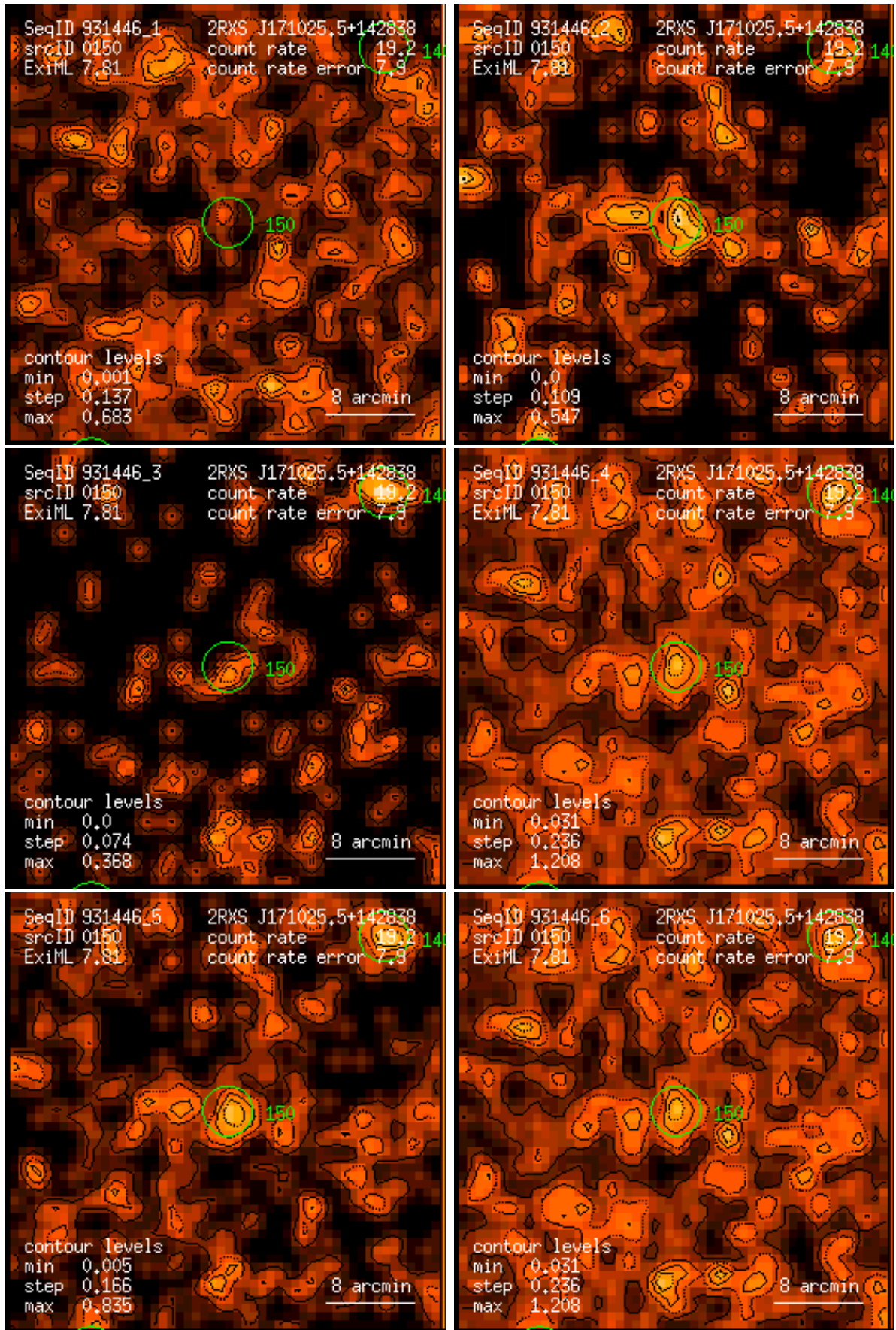
Figure 150: RASS 931446: detection 0150: band rate images, Gaussian filter: (1) PSPC channels 11 – 41, (2) 52 – 90, (3) 91 – 201, (4) 11 – 235, (5) 52 – 201, (6) 11 – 201. Broad band rates in counts/ks. Band rate contour levels in counts/ks/arcmin 2 .
