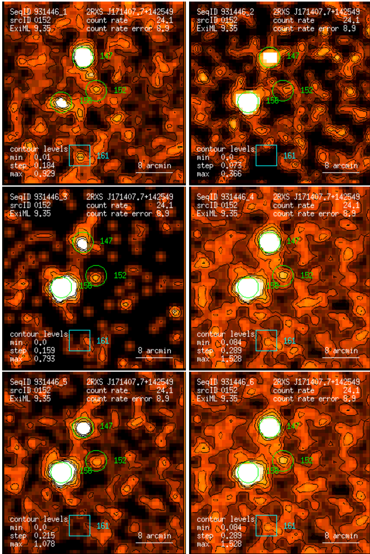
Figure 152: RASS 931446: detection 0152: band rate images, Gaussian filter: (1) PSPC channels 11 – 41, (2) 52 – 90, (3) 91 – 201, (4) 11 – 235, (5) 52 – 201, (6) 11 – 201. Broad band rates in counts/ks. Band rate contour levels in counts/ks/arcmin 2 .
