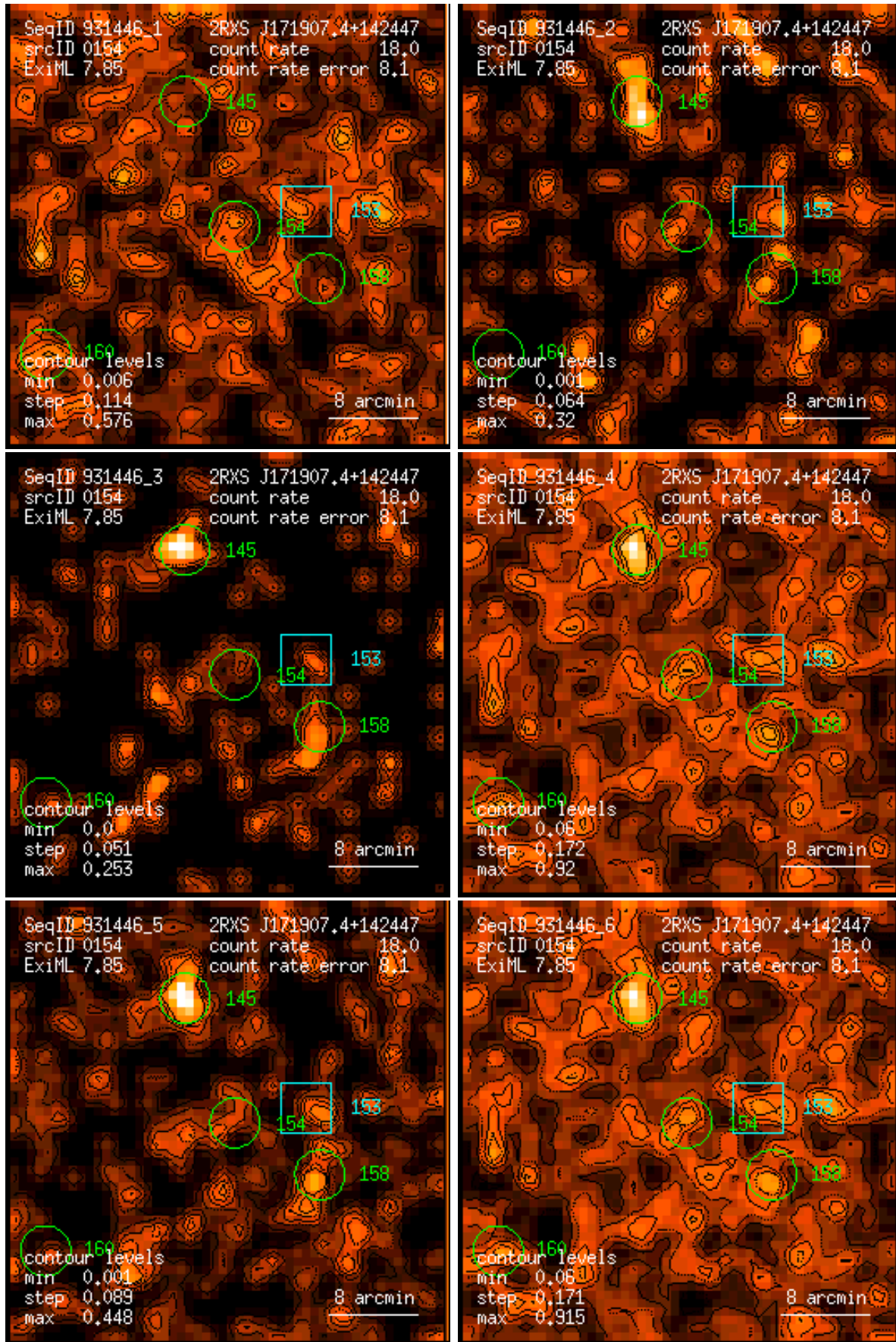
Figure 154: RASS 931446: detection 0154: band rate images, Gaussian filter: (1) PSPC channels 11 – 41, (2) 52 – 90, (3) 91 – 201, (4) 11 – 235, (5) 52 – 201, (6) 11 – 201. Broad band rates in counts/ks. Band rate contour levels in counts/ks/arcmin 2 .
